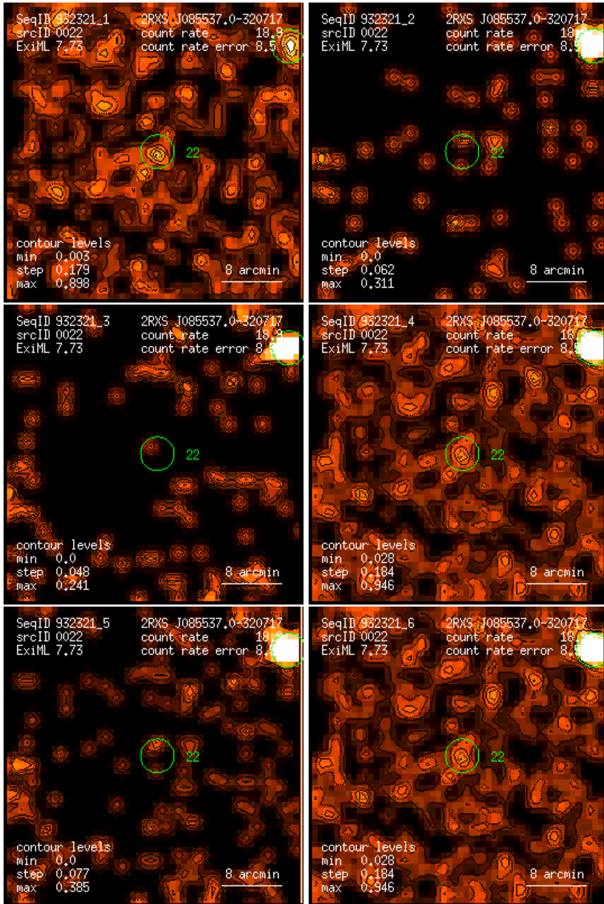
Figure 22: RASS 932321: detection 0022: band rate images, Gaussian filter: (1) PSPC channels 11 – 41, (2) 52 – 90, (3) 91 – 201, (4) 11 – 235, (5) 52 – 201, (6) 11 – 201. Broad band rates in counts/ks. Band rate contour levels in counts/ks/arcmin 2 .
