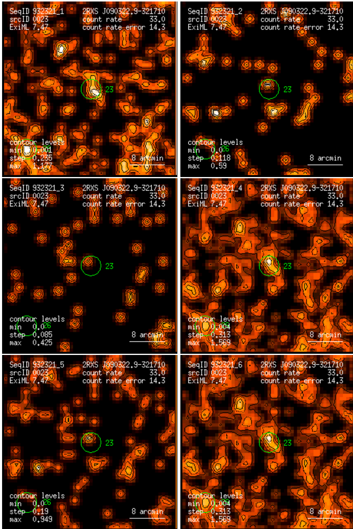
Figure 23: RASS 932321: detection 0023: band rate images, Gaussian filter: (1) PSPC channels 11 – 41, (2) 52 – 90, (3) 91 – 201, (4) 11 – 235, (5) 52 – 201, (6) 11 – 201. Broad band rates in counts/ks. Band rate contour levels in counts/ks/arcmin 2 .
