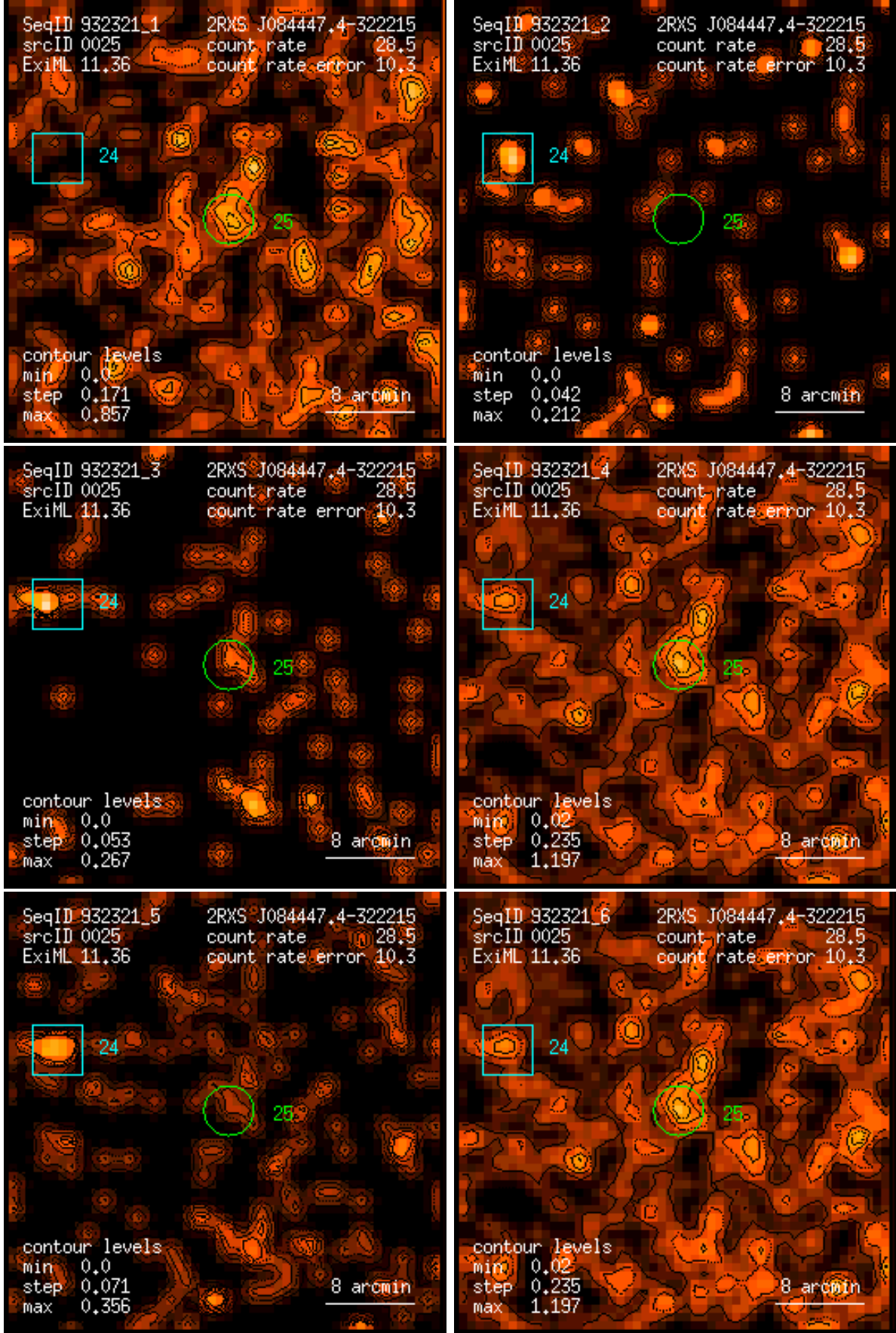
Figure 25: RASS 932321: detection 0025: band rate images, Gaussian filter: (1) PSPC channels 11 – 41, (2) 52 – 90, (3) 91 – 201, (4) 11 – 235, (5) 52 – 201, (6) 11 – 201. Broad band rates in counts/ks. Band rate contour levels in counts/ks/arcmin 2 .
