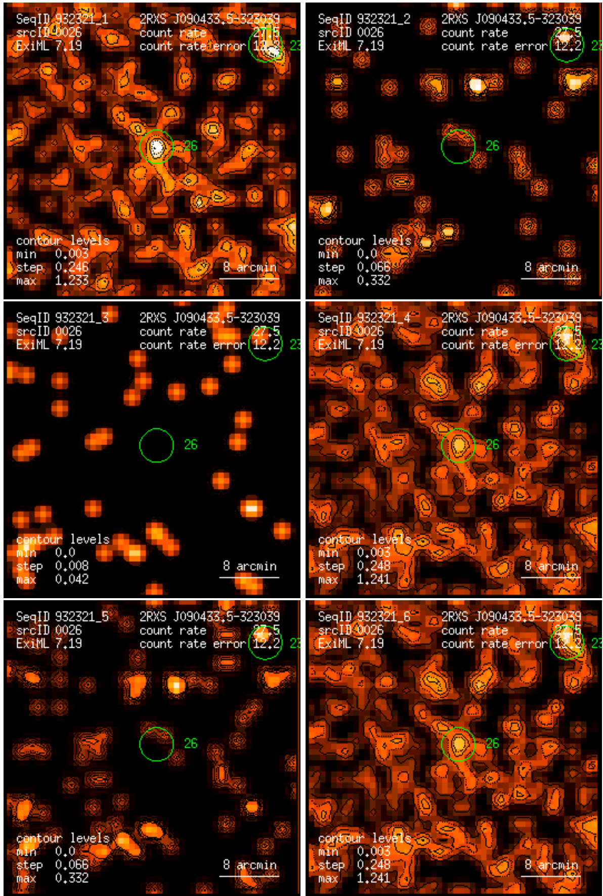
Figure 26: RASS 932321: detection 0026: band rate images, Gaussian filter: (1) PSPC channels 11 – 41, (2) 52 – 90, (3) 91 – 201, (4) 11 – 235, (5) 52 – 201, (6) 11 – 201. Broad band rates in counts/ks. Band rate contour levels in counts/ks/arcmin 2 .
