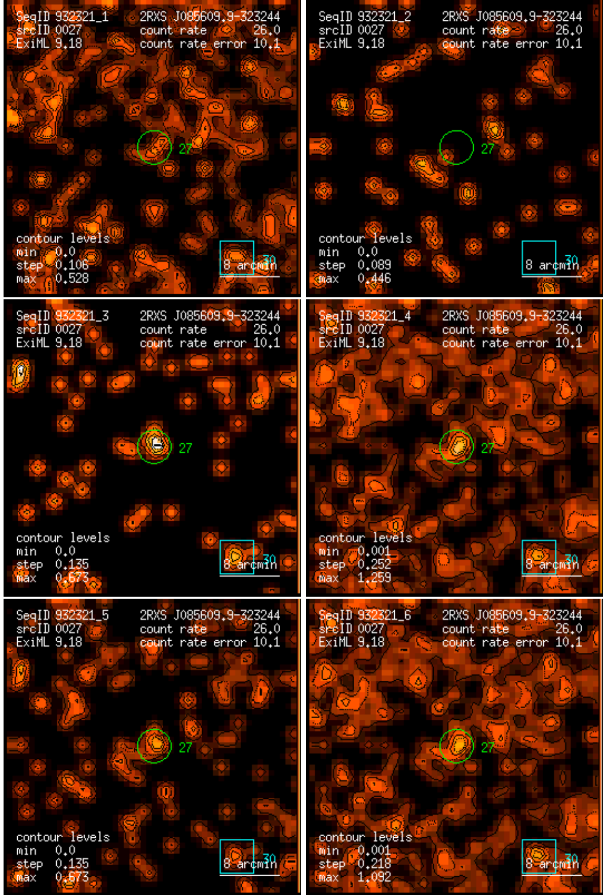
Figure 27: RASS 932321: detection 0027: band rate images, Gaussian filter: (1) PSPC channels 11 – 41, (2) 52 – 90, (3) 91 – 201, (4) 11 – 235, (5) 52 – 201, (6) 11 – 201. Broad band rates in counts/ks. Band rate contour levels in counts/ks/arcmin 2 .
