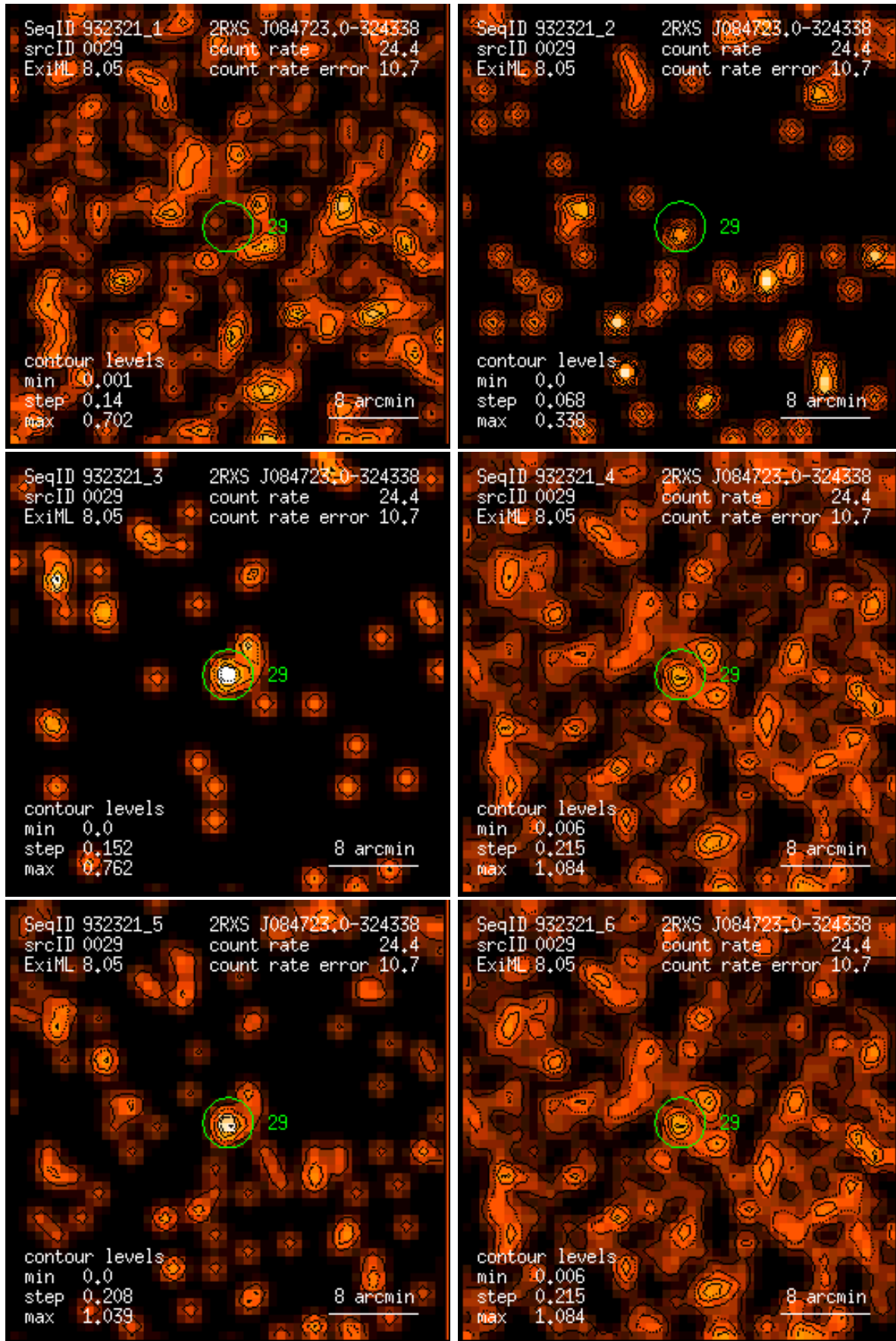
Figure 29: RASS 932321: detection 0029: band rate images, Gaussian filter: (1) PSPC channels 11 – 41, (2) 52 – 90, (3) 91 – 201, (4) 11 – 235, (5) 52 – 201, (6) 11 – 201. Broad band rates in counts/ks. Band rate contour levels in counts/ks/arcmin 2 .
