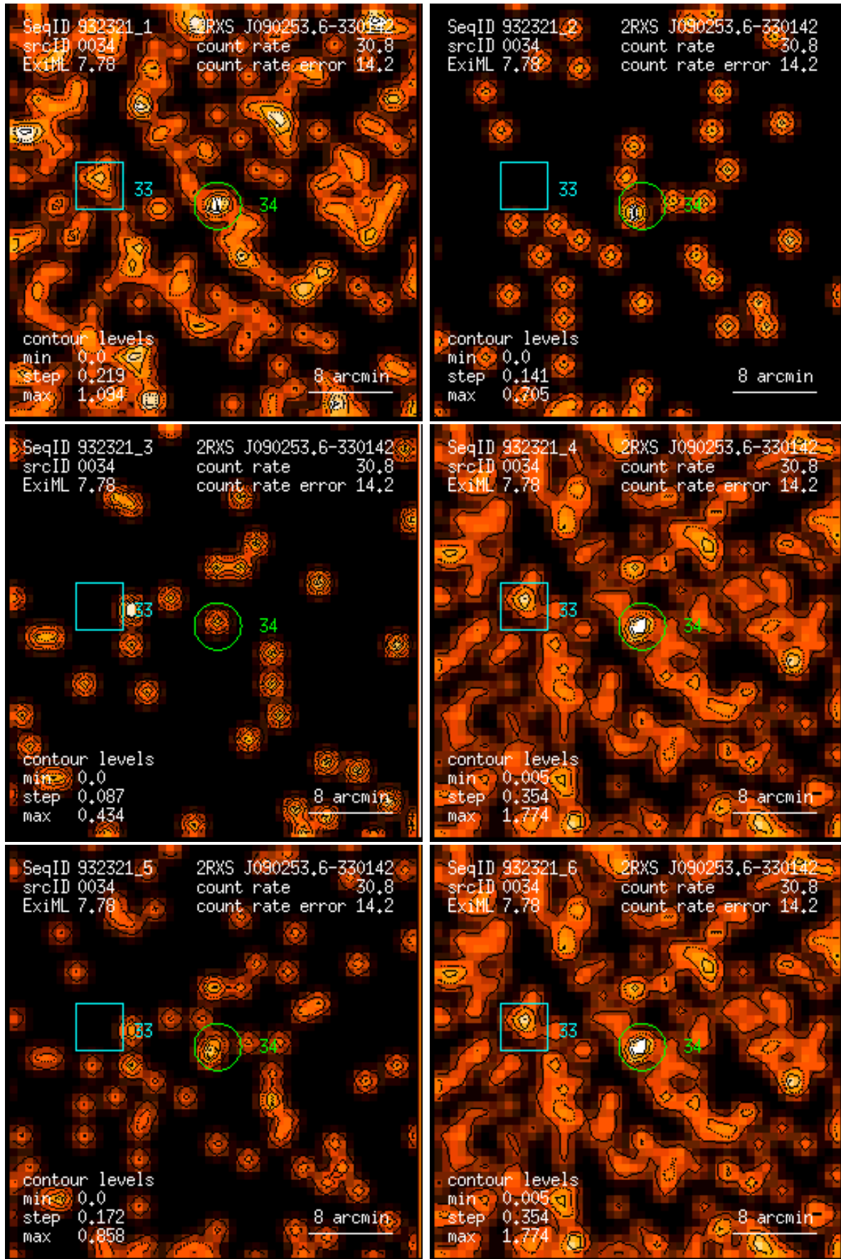
Figure 34: RASS 932321: detection 0034: band rate images, Gaussian filter: (1) PSPC channels 11 – 41, (2) 52 – 90, (3) 91 – 201, (4) 11 – 235, (5) 52 – 201, (6) 11 – 201. Broad band rates in counts/ks. Band rate contour levels in counts/ks/arcmin 2 .
