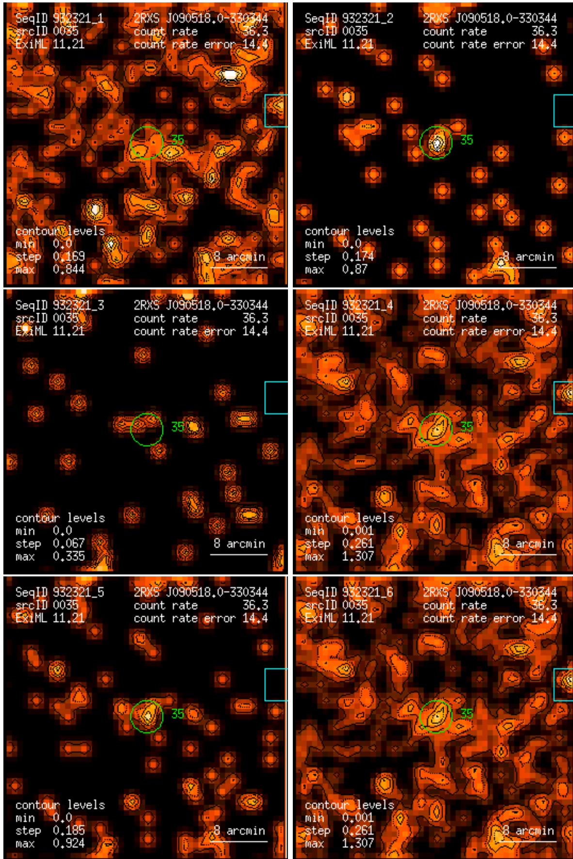
Figure 35: RASS 932321: detection 0035: band rate images, Gaussian filter: (1) PSPC channels 11 – 41, (2) 52 – 90, (3) 91 – 201, (4) 11 – 235, (5) 52 – 201, (6) 11 – 201. Broad band rates in counts/ks. Band rate contour levels in counts/ks/arcmin 2 .
