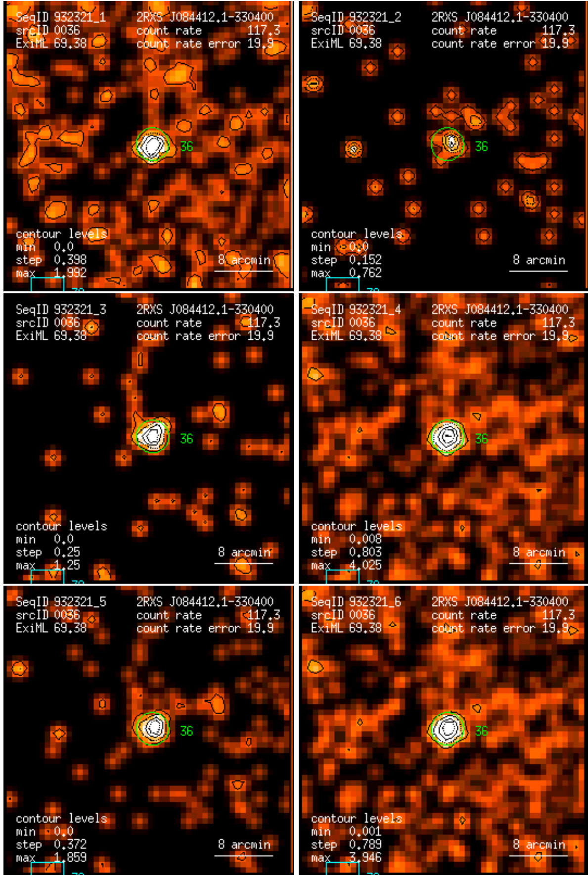
Figure 36: RASS 932321: detection 0036: band rate images, Gaussian filter: (1) PSPC channels 11 – 41, (2) 52 – 90, (3) 91 – 201, (4) 11 – 235, (5) 52 – 201, (6) 11 – 201. Broad band rates in counts/ks. Band rate contour levels in counts/ks/arcmin 2 .
