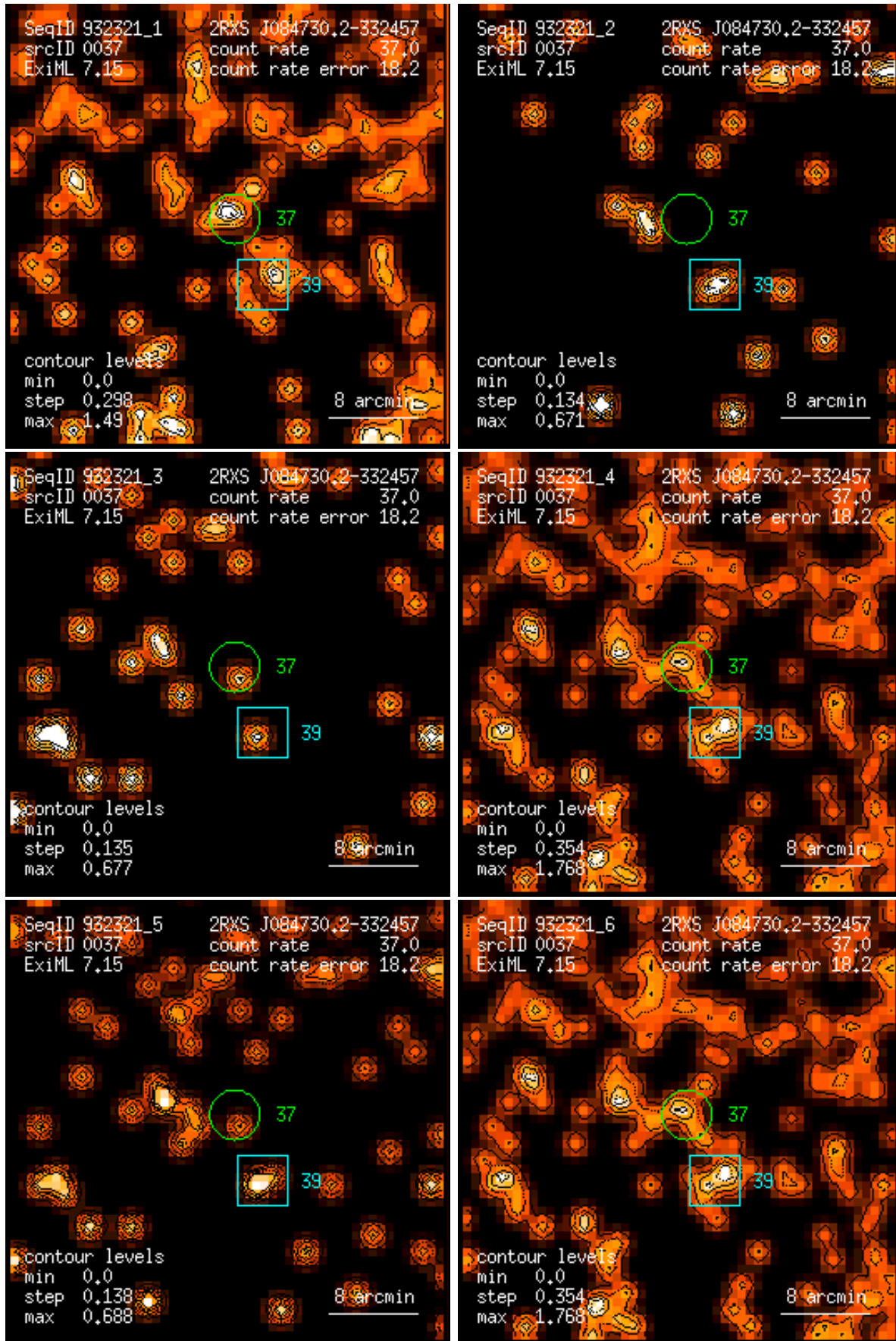
Figure 37: RASS 932321: detection 0037: band rate images, Gaussian filter: (1) PSPC channels 11 – 41, (2) 52 – 90, (3) 91 – 201, (4) 11 – 235, (5) 52 – 201, (6) 11 – 201. Broad band rates in counts/ks. Band rate contour levels in counts/ks/arcmin 2 .
