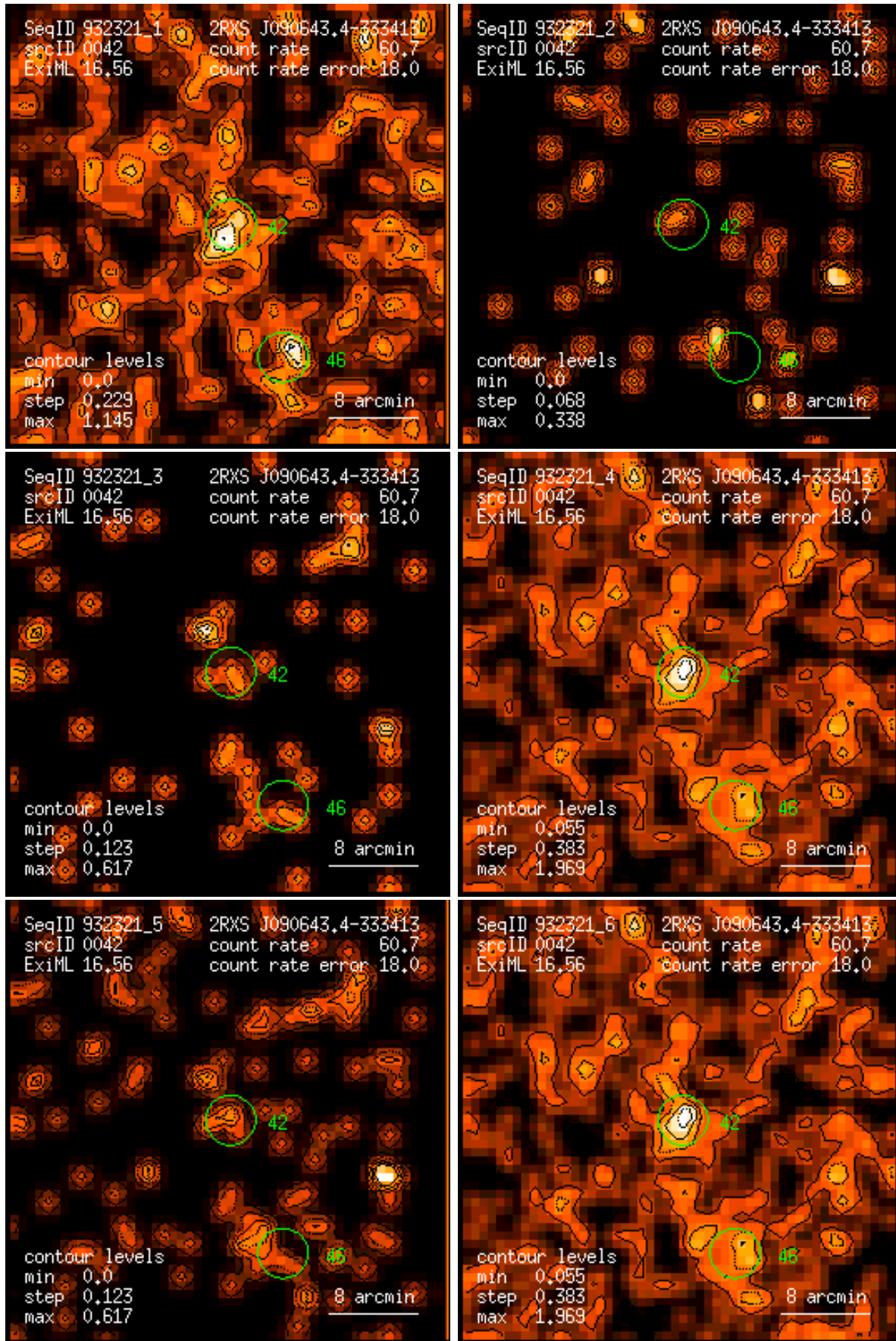
Figure 42: RASS 932321: detection 0042: band rate images, Gaussian filter: (1) PSPC channels 11 – 41, (2) 52 – 90, (3) 91 – 201, (4) 11 – 235, (5) 52 – 201, (6) 11 – 201. Broad band rates in counts/ks. Band rate contour levels in counts/ks/arcmin 2 .
