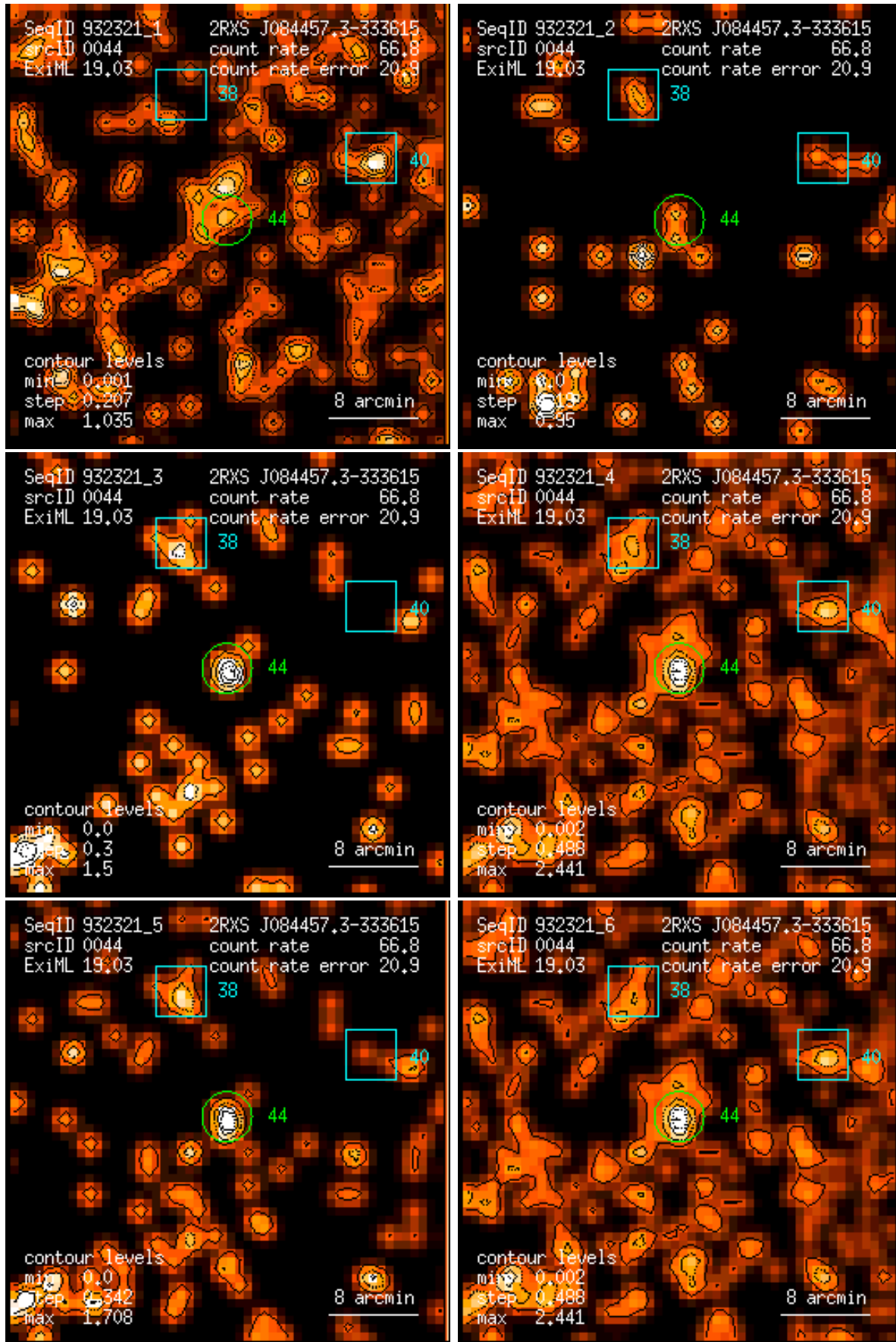
Figure 44: RASS 932321: detection 0044: band rate images, Gaussian filter: (1) PSPC channels 11 – 41, (2) 52 – 90, (3) 91 – 201, (4) 11 – 235, (5) 52 – 201, (6) 11 – 201. Broad band rates in counts/ks. Band rate contour levels in counts/ks/arcmin 2 .
