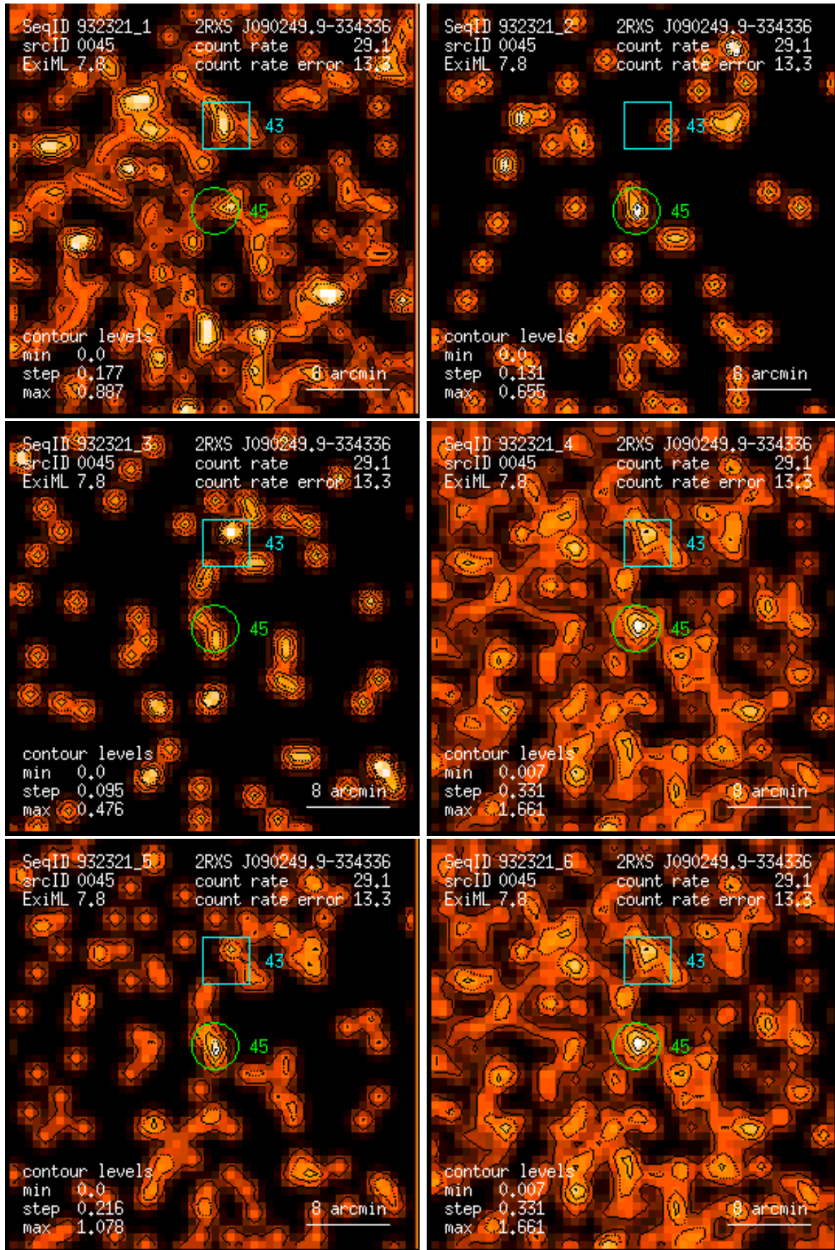
Figure 45: RASS 932321: detection 0045: band rate images, Gaussian filter: (1) PSPC channels 11 – 41, (2) 52 – 90, (3) 91 – 201, (4) 11 – 235, (5) 52 – 201, (6) 11 – 201. Broad band rates in counts/ks. Band rate contour levels in counts/ks/arcmin 2 .
