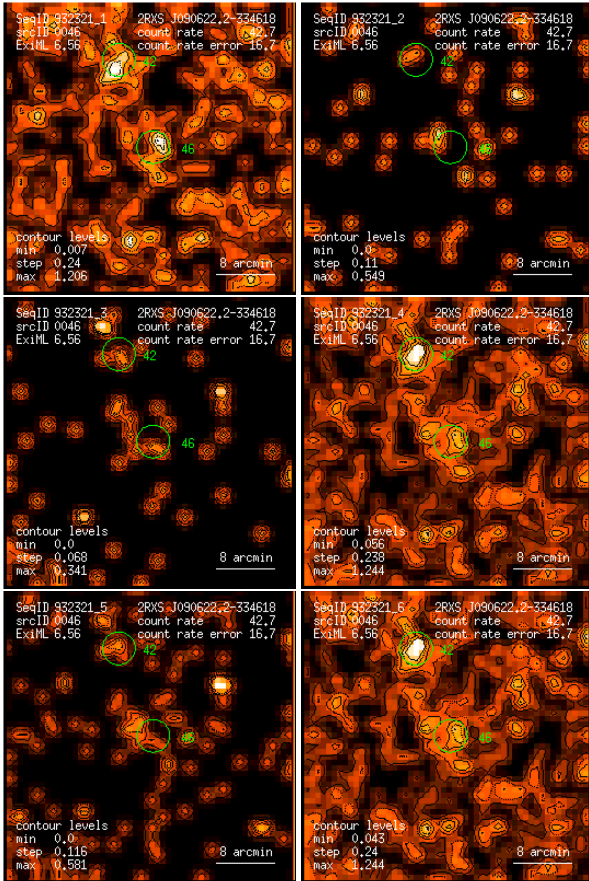
Figure 46: RASS 932321: detection 0046: band rate images, Gaussian filter: (1) PSPC channels 11 – 41, (2) 52 – 90, (3) 91 – 201, (4) 11 – 235, (5) 52 – 201, (6) 11 – 201. Broad band rates in counts/ks. Band rate contour levels in counts/ks/arcmin 2 .
