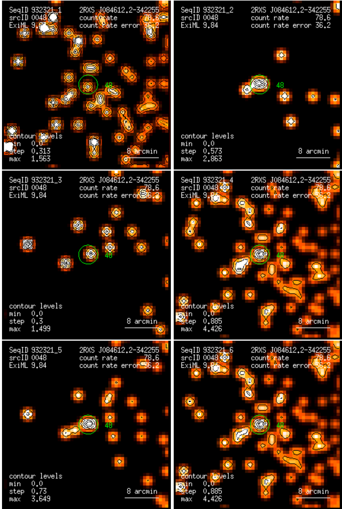
Figure 48: RASS 932321: detection 0048: band rate images, Gaussian filter: (1) PSPC channels 11 – 41, (2) 52 – 90, (3) 91 – 201, (4) 11 – 235, (5) 52 – 201, (6) 11 – 201. Broad band rates in counts/ks. Band rate contour levels in counts/ks/arcmin 2 .
