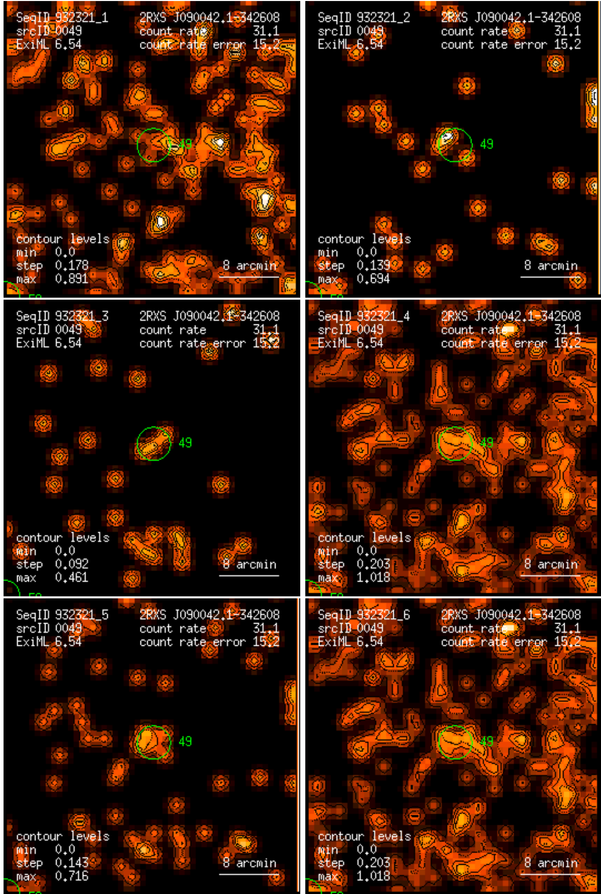
Figure 49: RASS 932321: detection 0049: band rate images, Gaussian filter: (1) PSPC channels 11 – 41, (2) 52 – 90, (3) 91 – 201, (4) 11 – 235, (5) 52 – 201, (6) 11 – 201. Broad band rates in counts/ks. Band rate contour levels in counts/ks/arcmin 2 .
