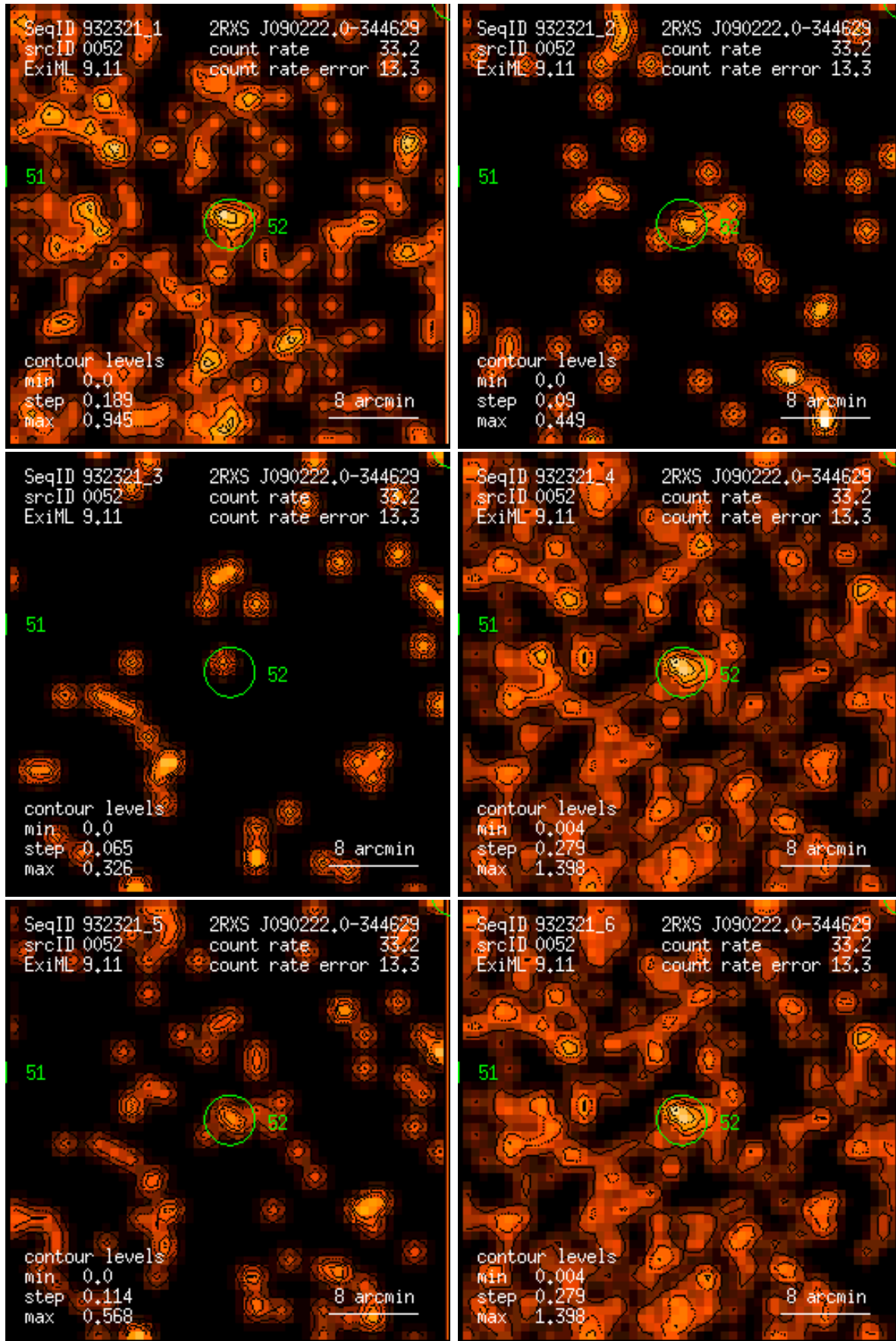
Figure 52: RASS 932321: detection 0052: band rate images, Gaussian filter: (1) PSPC channels 11 – 41, (2) 52 – 90, (3) 91 – 201, (4) 11 – 235, (5) 52 – 201, (6) 11 – 201. Broad band rates in counts/ks. Band rate contour levels in counts/ks/arcmin 2 .
