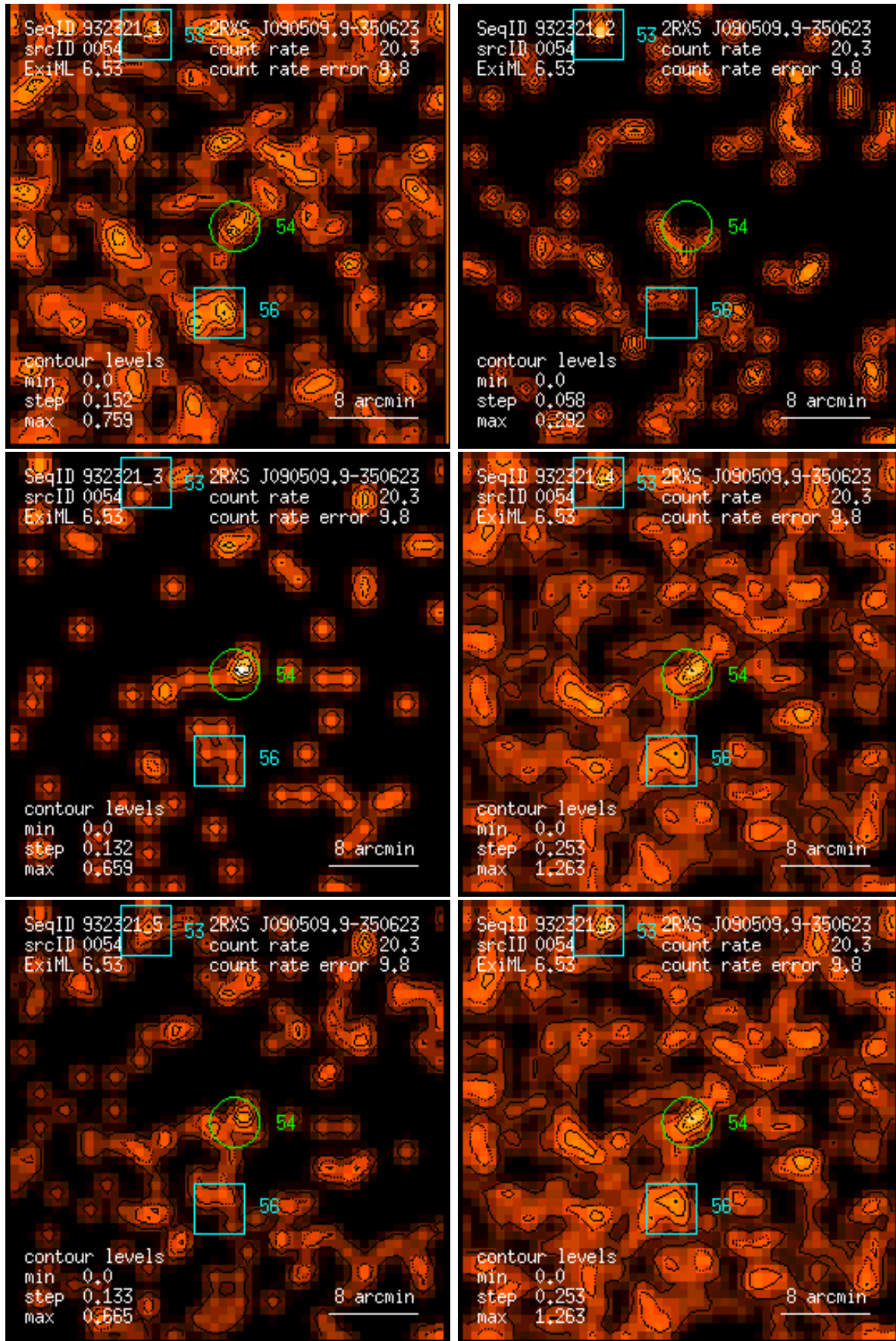
Figure 54: RASS 932321: detection 0054: band rate images, Gaussian filter: (1) PSPC channels 11 – 41, (2) 52 – 90, (3) 91 – 201, (4) 11 – 235, (5) 52 – 201, (6) 11 – 201. Broad band rates in counts/ks. Band rate contour levels in counts/ks/arcmin 2 .
