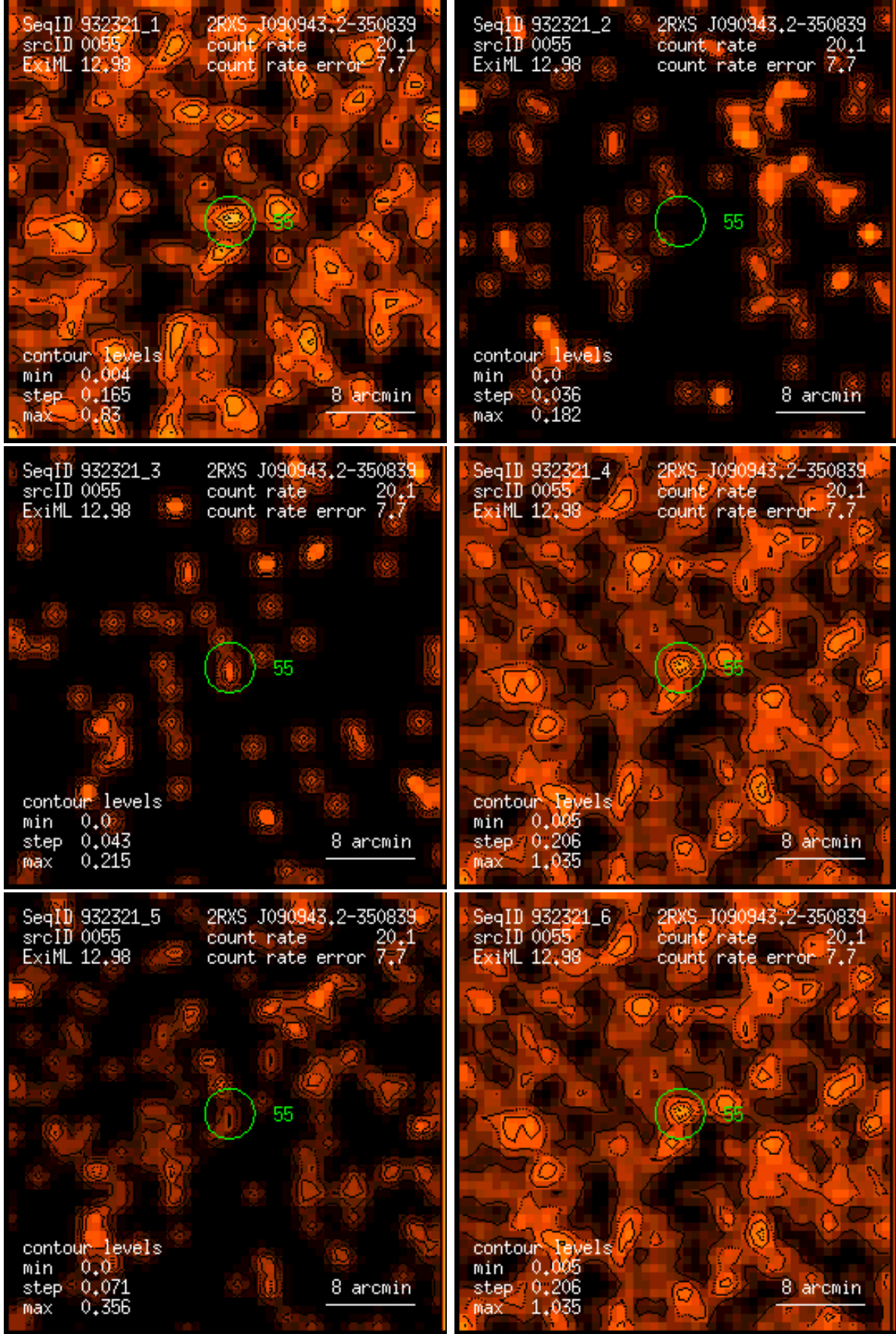
Figure 55: RASS 932321: detection 0055: band rate images, Gaussian filter: (1) PSPC channels 11 – 41, (2) 52 – 90, (3) 91 – 201, (4) 11 – 235, (5) 52 – 201, (6) 11 – 201. Broad band rates in counts/ks. Band rate contour levels in counts/ks/arcmin 2 .
