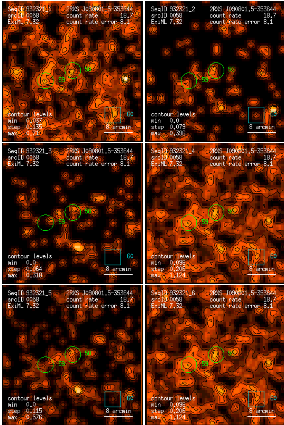
Figure 58: RASS 932321: detection 0058: band rate images, Gaussian filter: (1) PSPC channels 11 – 41, (2) 52 – 90, (3) 91 – 201, (4) 11 – 235, (5) 52 – 201, (6) 11 – 201. Broad band rates in counts/ks. Band rate contour levels in counts/ks/arcmin 2 .
