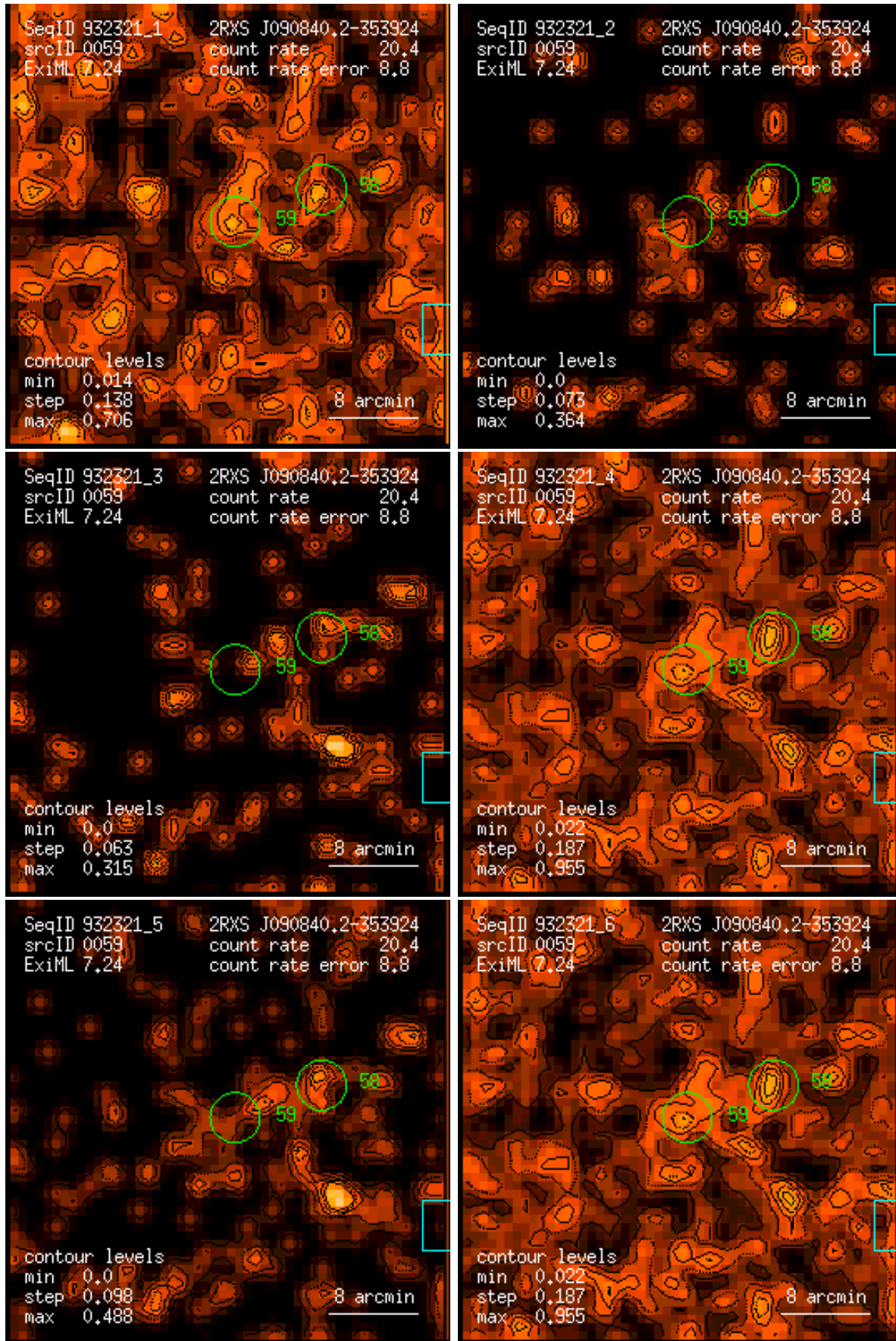
Figure 59: RASS 932321: detection 0059: band rate images, Gaussian filter: (1) PSPC channels 11 – 41, (2) 52 – 90, (3) 91 – 201, (4) 11 – 235, (5) 52 – 201, (6) 11 – 201. Broad band rates in counts/ks. Band rate contour levels in counts/ks/arcmin 2 .
