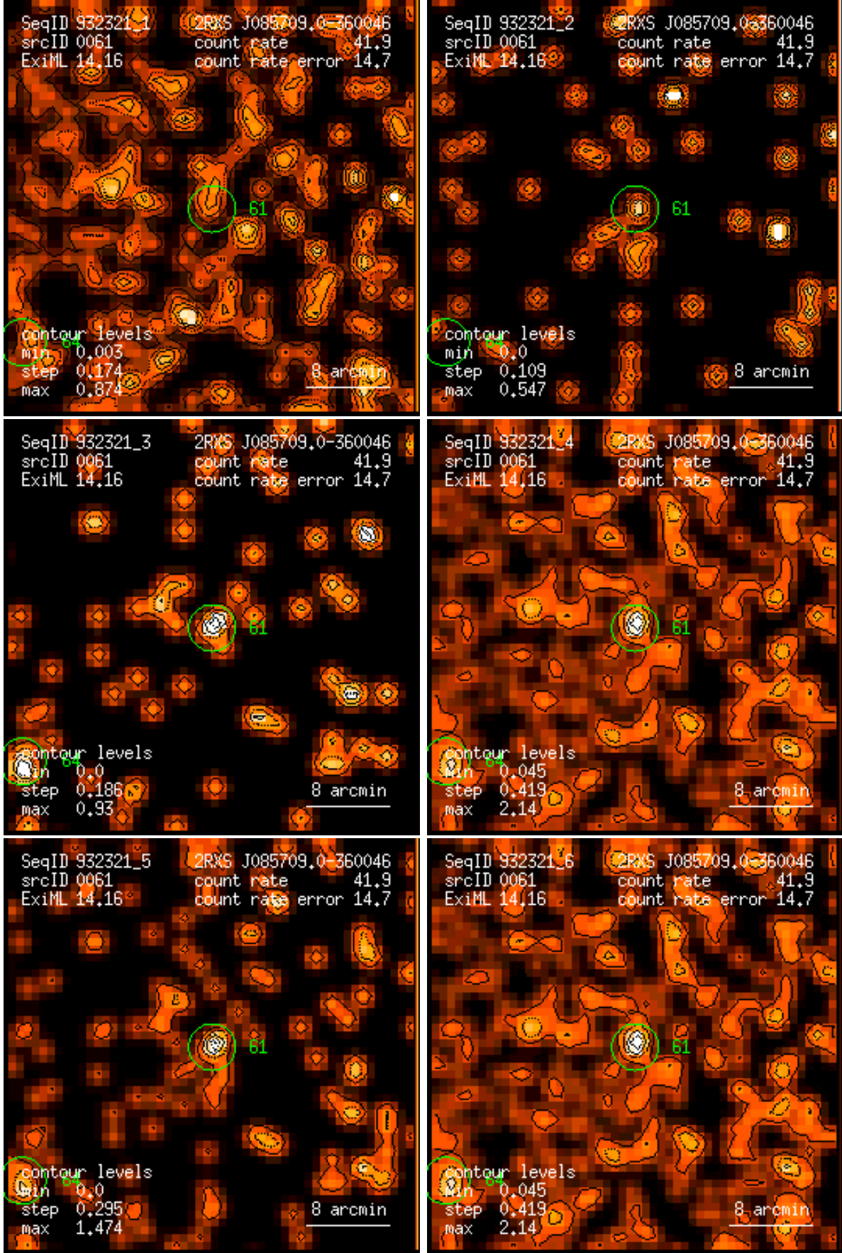
Figure 61: RASS 932321: detection 0061: band rate images, Gaussian filter: (1) PSPC channels 11 – 41, (2) 52 – 90, (3) 91 – 201, (4) 11 – 235, (5) 52 – 201, (6) 11 – 201. Broad band rates in counts/ks. Band rate contour levels in counts/ks/arcmin 2 .
