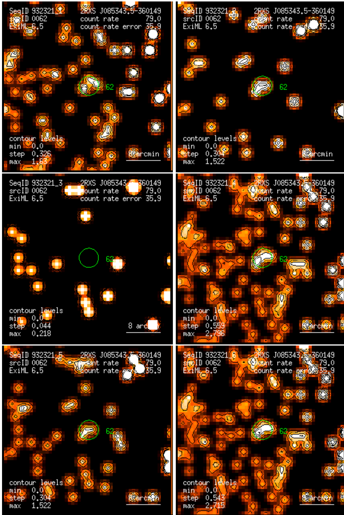
Figure 62: RASS 932321: detection 0062: band rate images, Gaussian filter: (1) PSPC channels 11 – 41, (2) 52 – 90, (3) 91 – 201, (4) 11 – 235, (5) 52 – 201, (6) 11 – 201. Broad band rates in counts/ks. Band rate contour levels in counts/ks/arcmin 2 .
