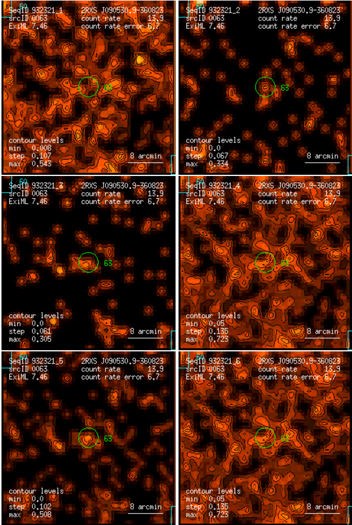
Figure 63: RASS 932321: detection 0063: band rate images, Gaussian filter: (1) PSPC channels 11 – 41, (2) 52 – 90, (3) 91 – 201, (4) 11 – 235, (5) 52 – 201, (6) 11 – 201. Broad band rates in counts/ks. Band rate contour levels in counts/ks/arcmin 2 .
