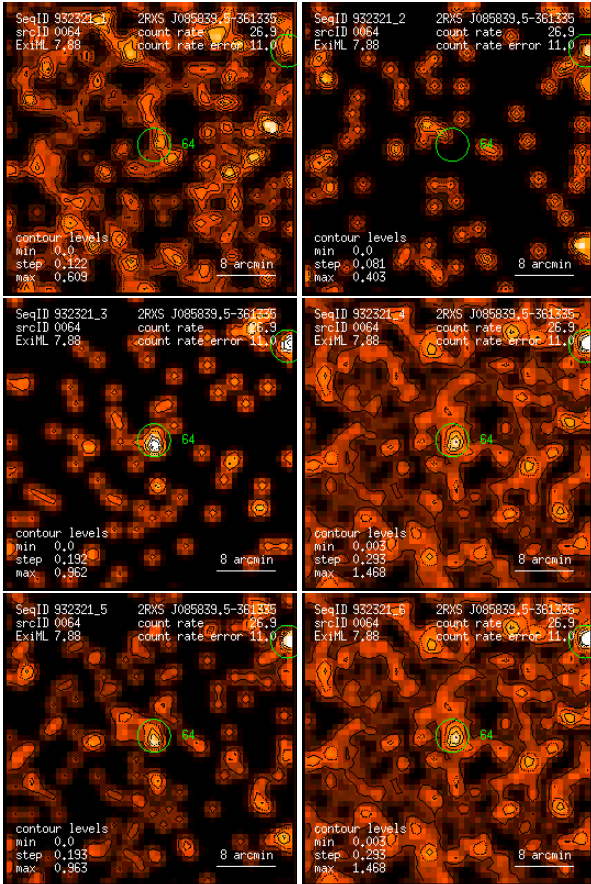
Figure 64: RASS 932321: detection 0064: band rate images, Gaussian filter: (1) PSPC channels 11 – 41, (2) 52 – 90, (3) 91 – 201, (4) 11 – 235, (5) 52 – 201, (6) 11 – 201. Broad band rates in counts/ks. Band rate contour levels in counts/ks/arcmin 2 .
