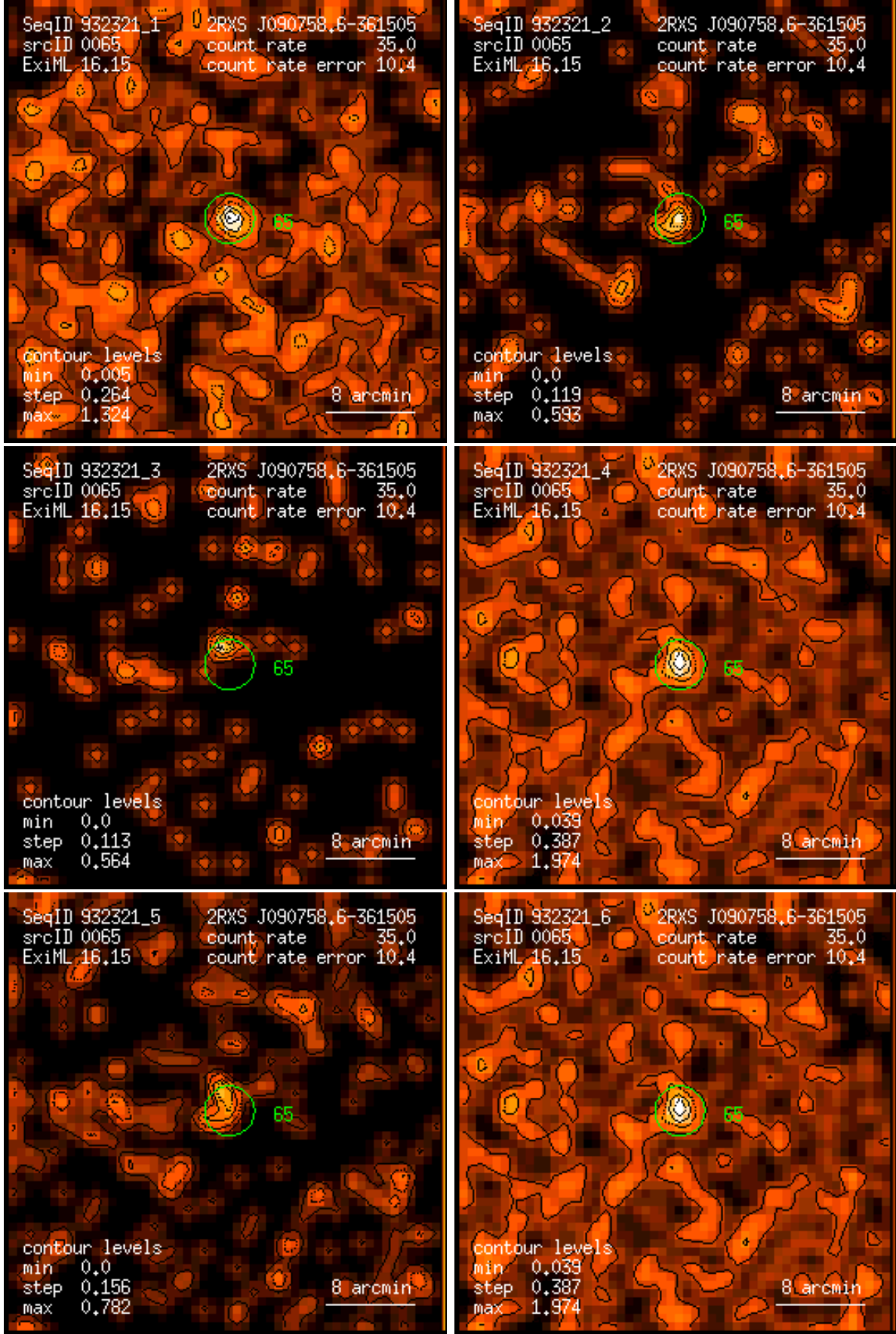
Figure 65: RASS 932321: detection 0065: band rate images, Gaussian filter: (1) PSPC channels 11 – 41, (2) 52 – 90, (3) 91 – 201, (4) 11 – 235, (5) 52 – 201, (6) 11 – 201. Broad band rates in counts/ks. Band rate contour levels in counts/ks/arcmin 2 .
