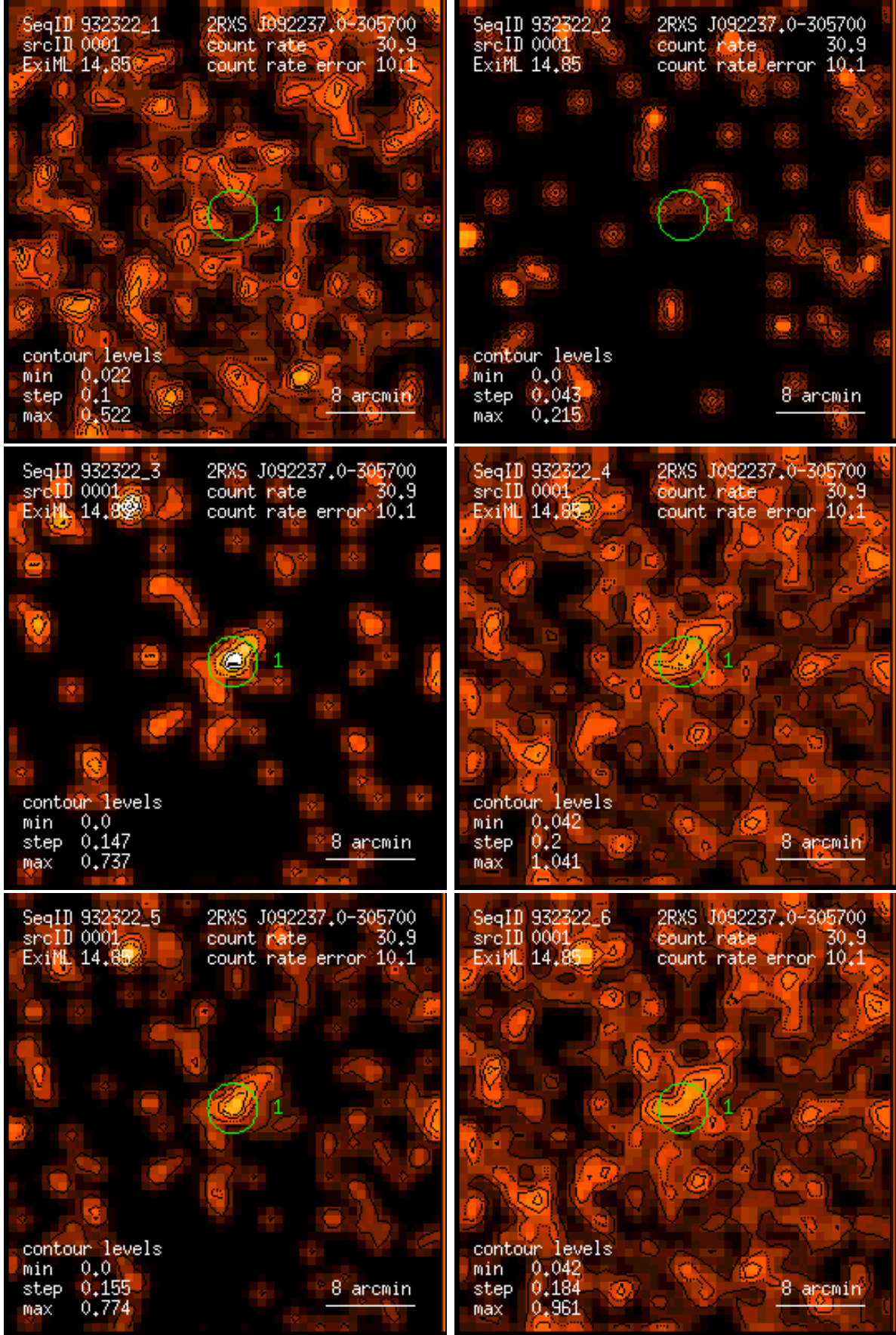
Figure 1: RASS 932322: detection 0001: band rate images, Gaussian filter: (1) PSPC channels 11 – 41, (2) 52 – 90, (3) 91 – 201, (4) 11 – 235, (5) 52 – 201, (6) 11 – 201. Broad band rates in counts/ks. Band rate contour levels in counts/ks/arcmin 2 .
