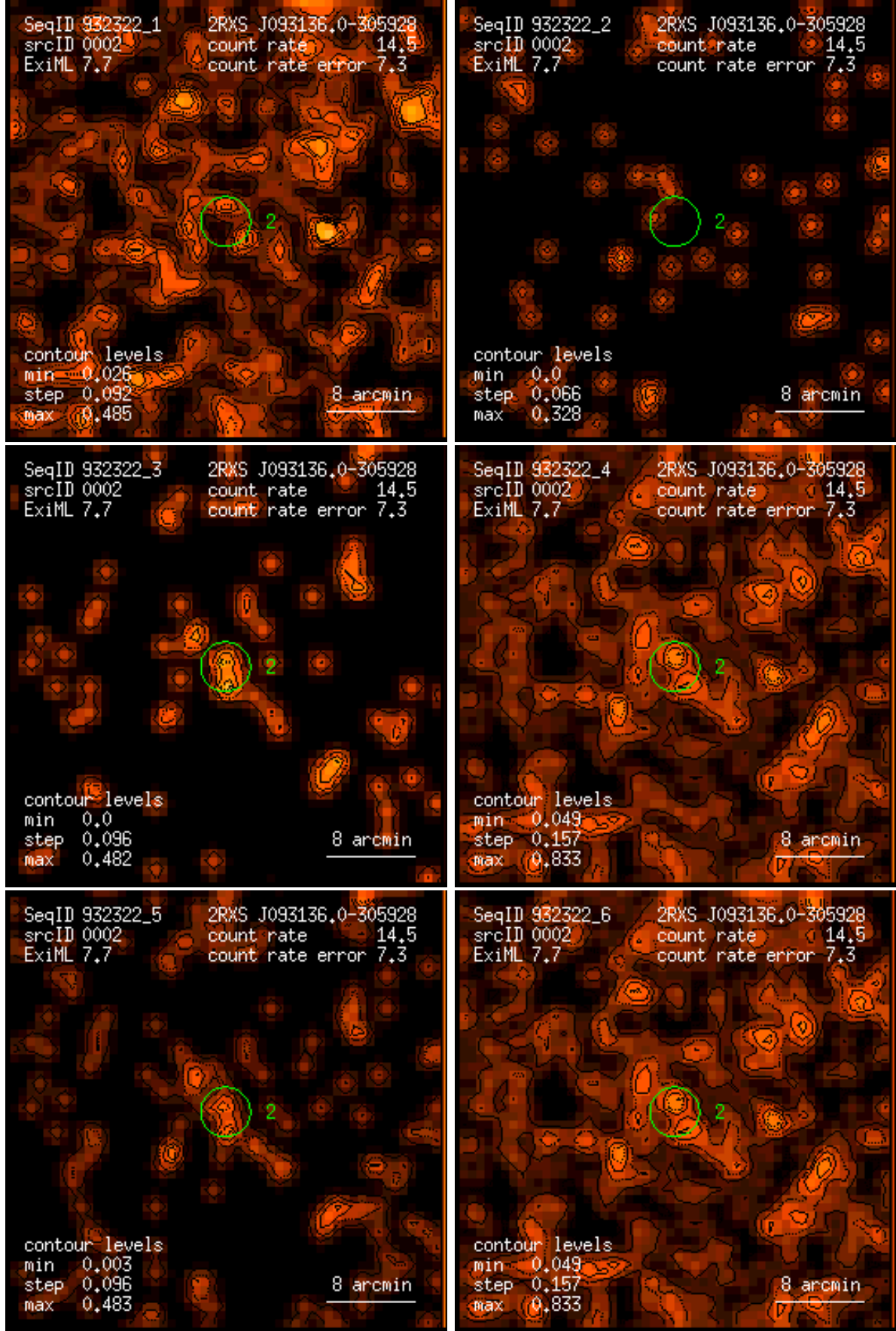
Figure 2: RASS 932322: detection 0002: band rate images, Gaussian filter: (1) PSPC channels 11 – 41, (2) 52 – 90, (3) 91 – 201, (4) 11 – 235, (5) 52 – 201, (6) 11 – 201. Broad band rates in counts/ks. Band rate contour levels in counts/ks/arcmin 2 .
