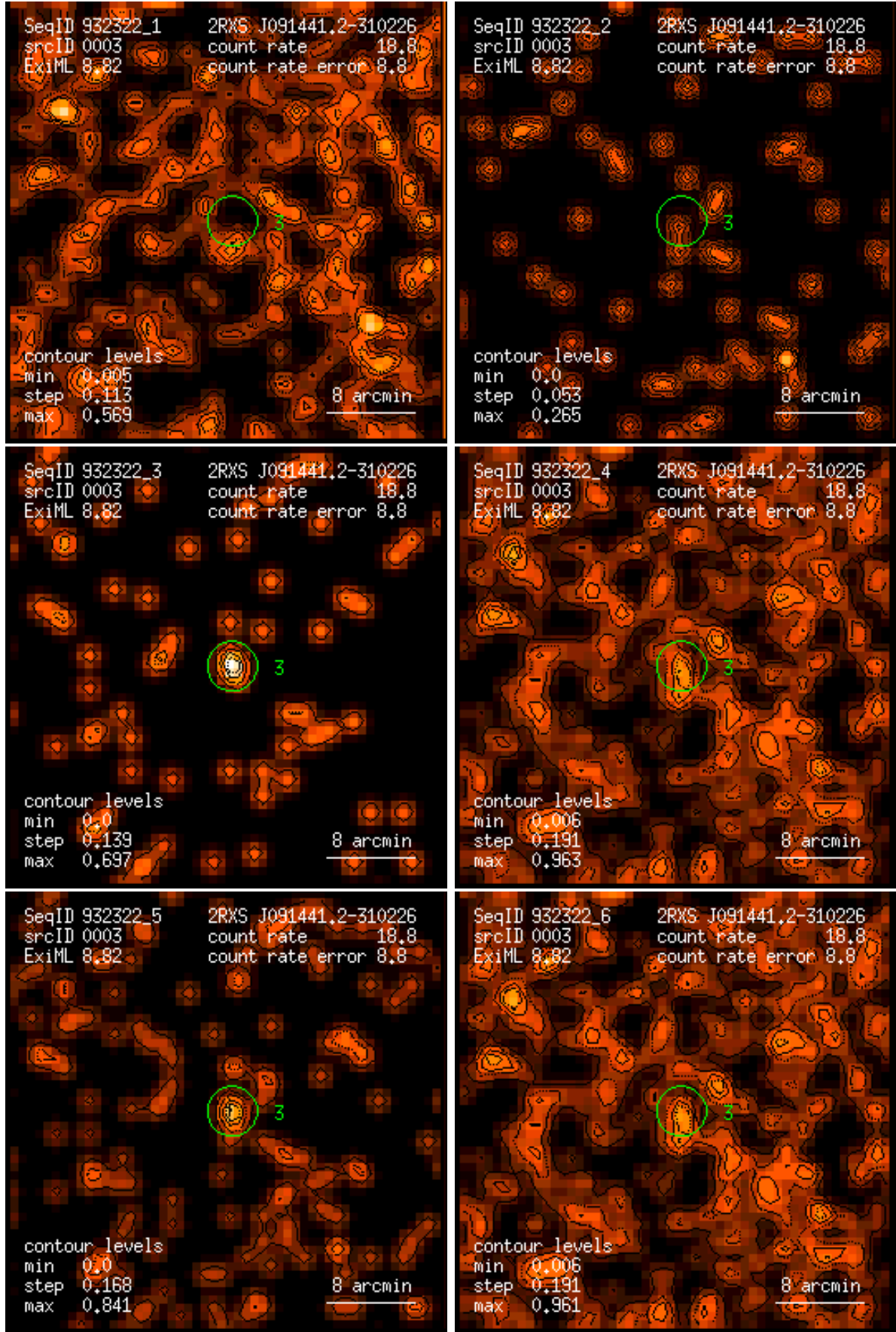
Figure 3: RASS 932322: detection 0003: band rate images, Gaussian filter: (1) PSPC channels 11 – 41, (2) 52 – 90, (3) 91 – 201, (4) 11 – 235, (5) 52 – 201, (6) 11 – 201. Broad band rates in counts/ks. Band rate contour levels in counts/ks/arcmin 2 .
