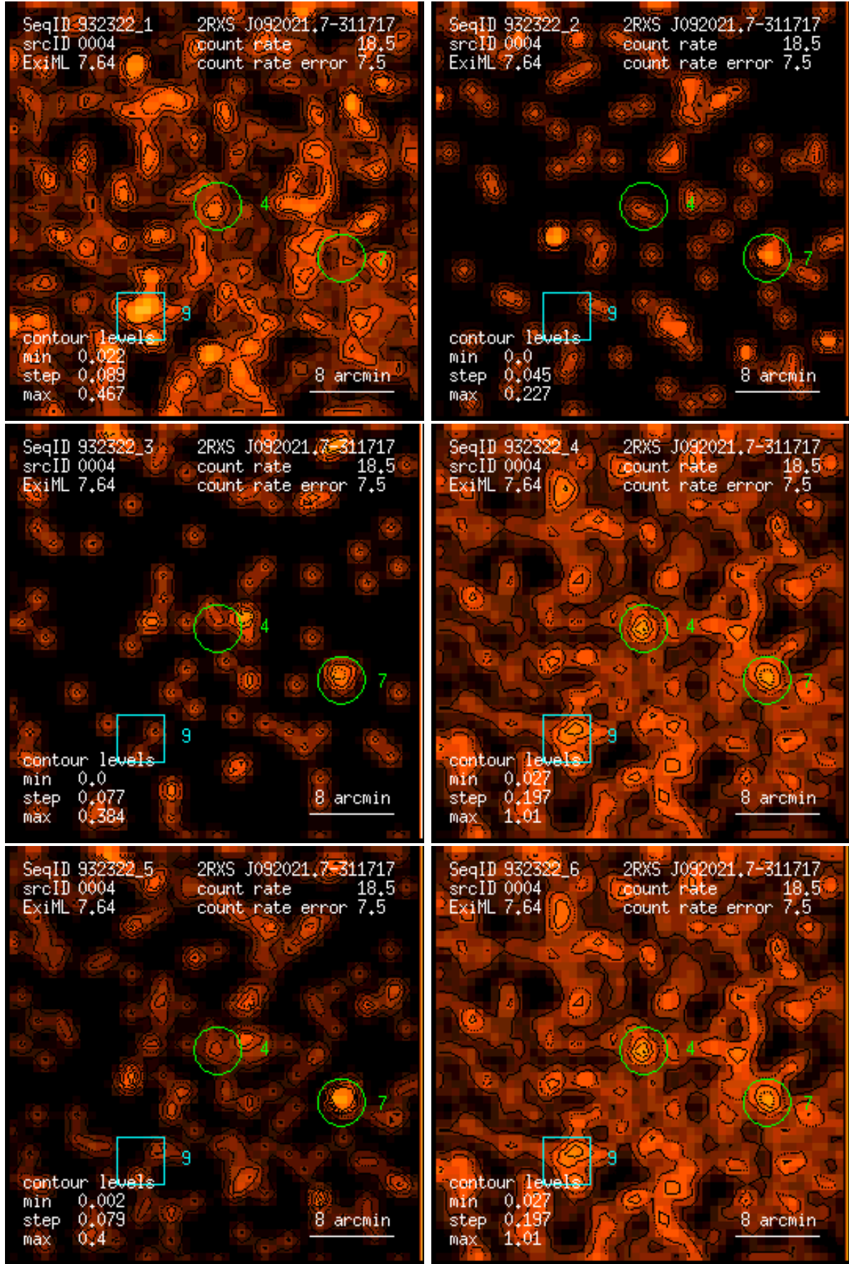
Figure 4: RASS 932322: detection 0004: band rate images, Gaussian filter: (1) PSPC channels 11 – 41, (2) 52 – 90, (3) 91 – 201, (4) 11 – 235, (5) 52 – 201, (6) 11 – 201. Broad band rates in counts/ks. Band rate contour levels in counts/ks/arcmin 2 .
