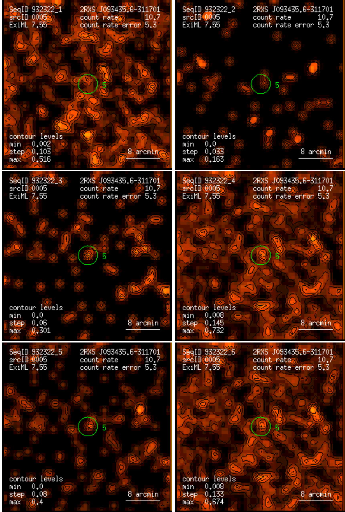
Figure 5: RASS 932322: detection 0005: band rate images, Gaussian filter: (1) PSPC channels 11 – 41, (2) 52 – 90, (3) 91 – 201, (4) 11 – 235, (5) 52 – 201, (6) 11 – 201. Broad band rates in counts/ks. Band rate contour levels in counts/ks/arcmin 2 .
