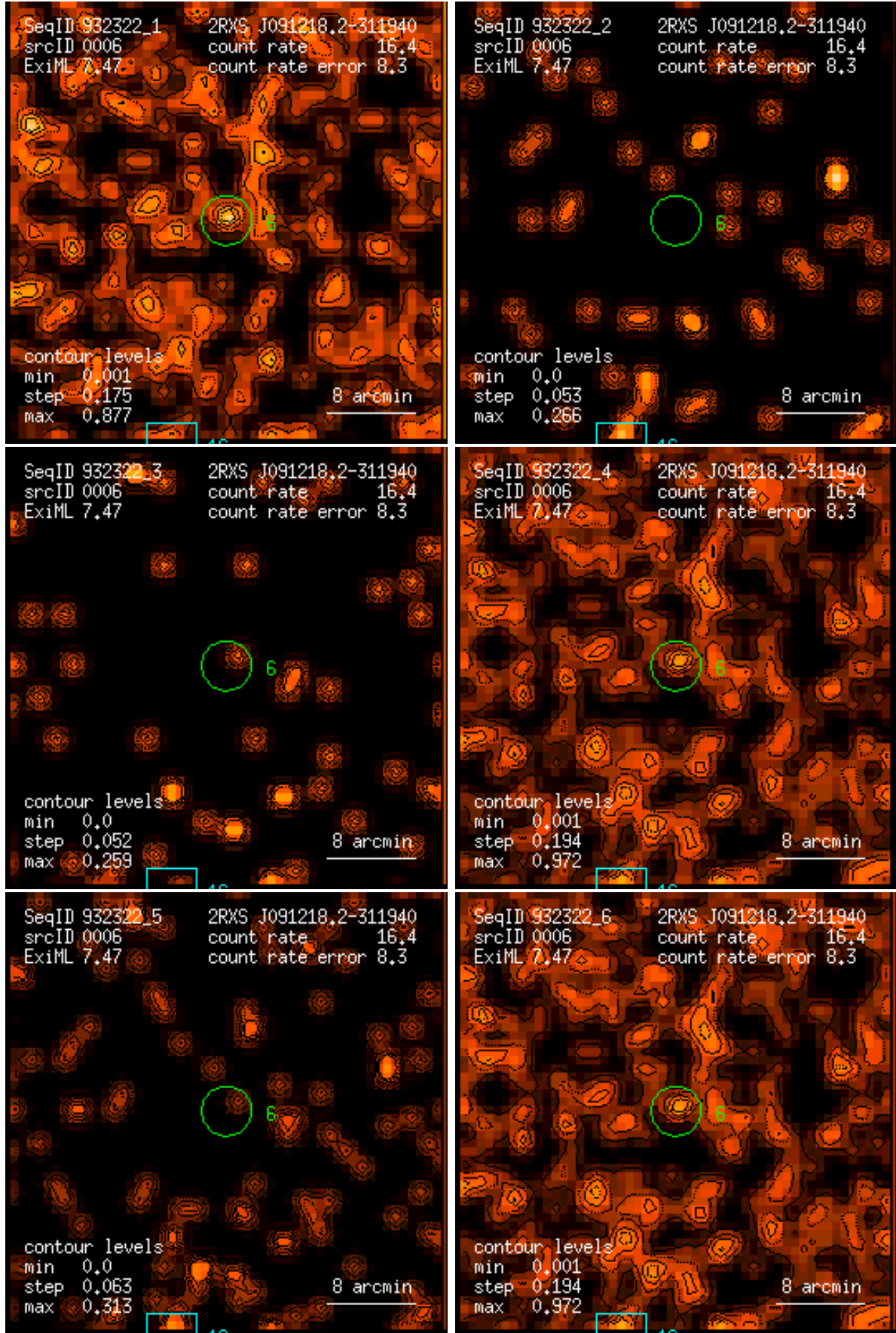
Figure 6: RASS 932322: detection 0006: band rate images, Gaussian filter: (1) PSPC channels 11 – 41, (2) 52 – 90, (3) 91 – 201, (4) 11 – 235, (5) 52 – 201, (6) 11 – 201. Broad band rates in counts/ks. Band rate contour levels in counts/ks/arcmin 2 .
