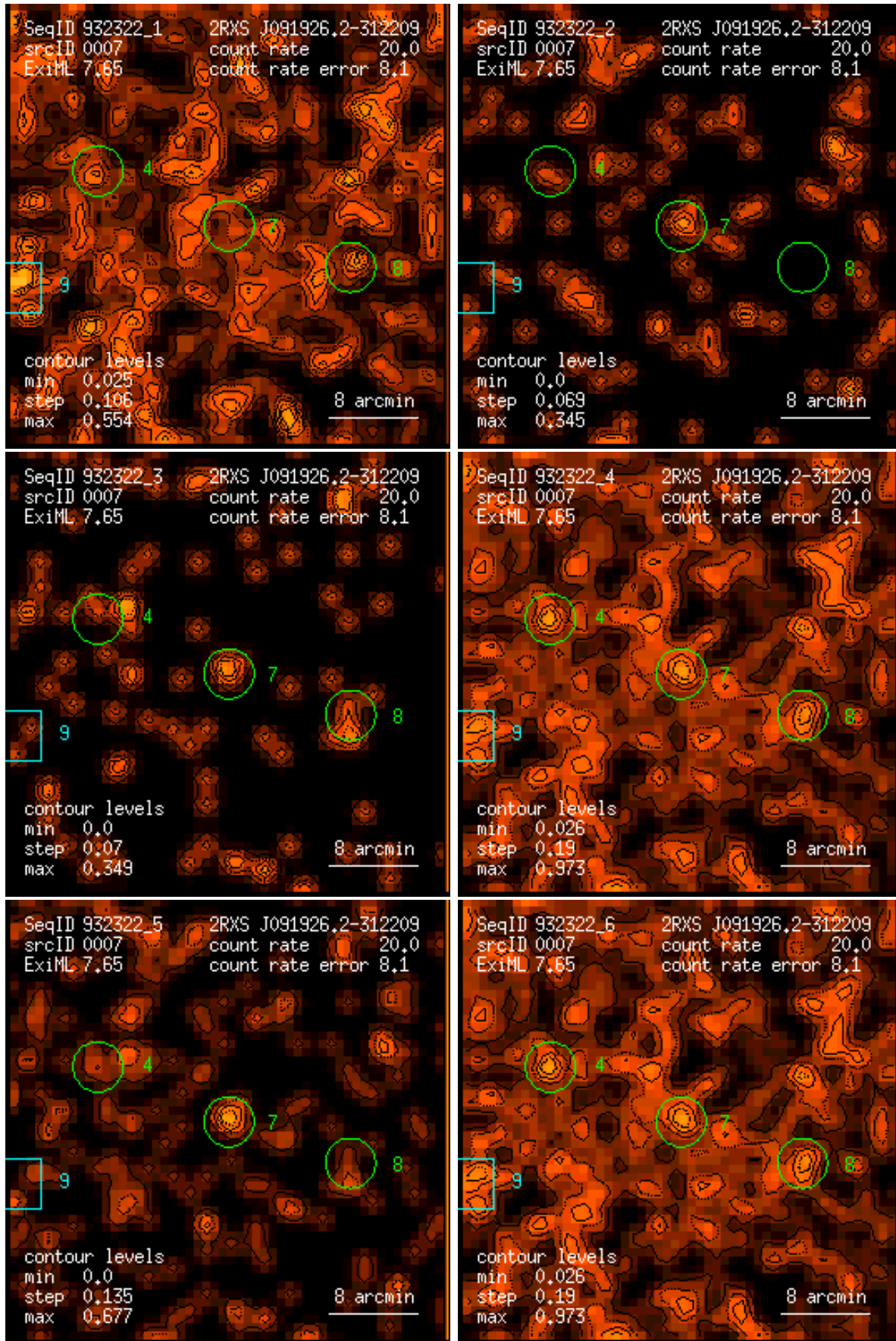
Figure 7: RASS 932322: detection 0007: band rate images, Gaussian filter: (1) PSPC channels 11 – 41, (2) 52 – 90, (3) 91 – 201, (4) 11 – 235, (5) 52 – 201, (6) 11 – 201. Broad band rates in counts/ks. Band rate contour levels in counts/ks/arcmin 2 .
