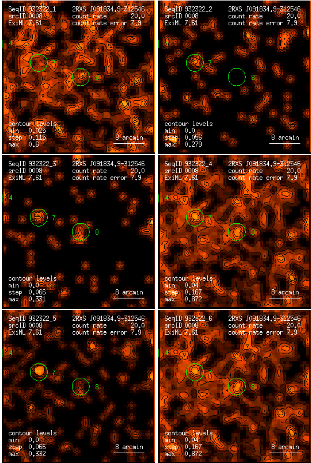
Figure 8: RASS 932322: detection 0008: band rate images, Gaussian filter: (1) PSPC channels 11 – 41, (2) 52 – 90, (3) 91 – 201, (4) 11 – 235, (5) 52 – 201, (6) 11 – 201. Broad band rates in counts/ks. Band rate contour levels in counts/ks/arcmin 2 .
