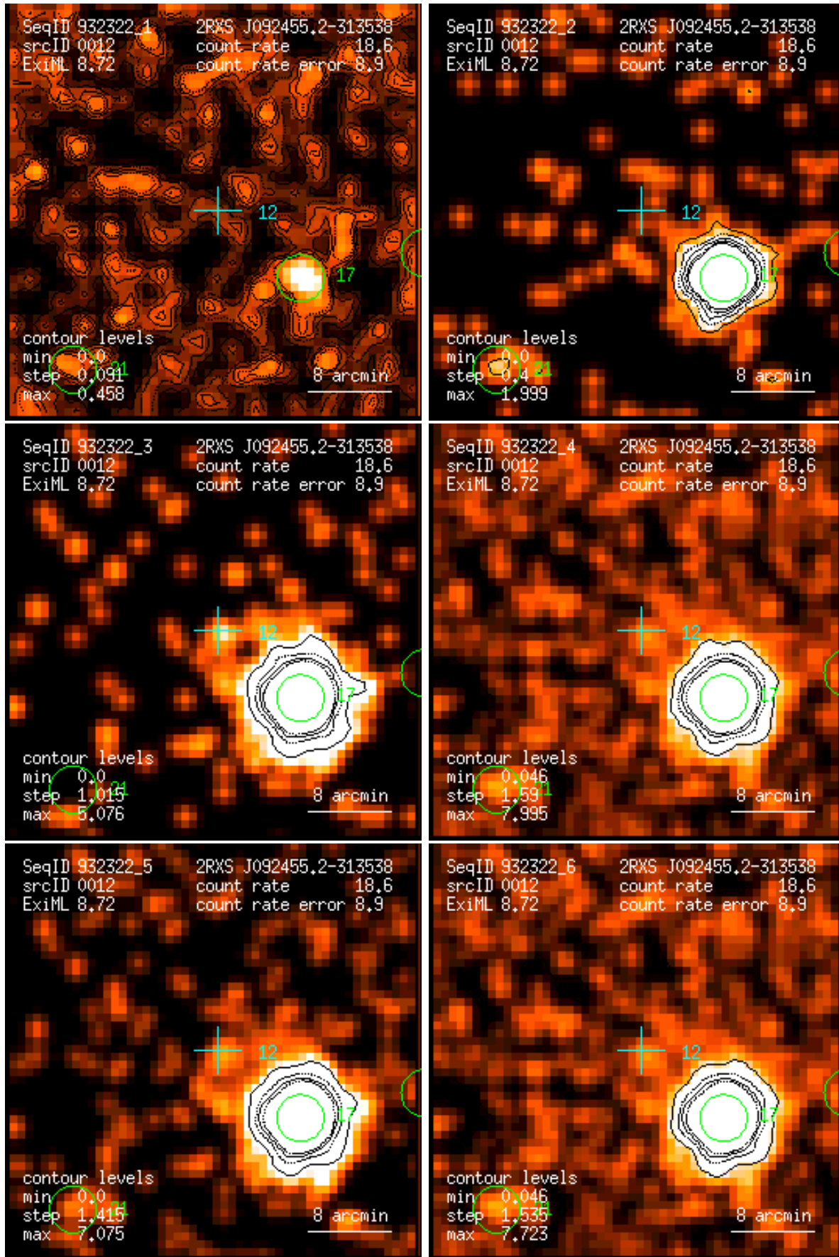
Figure 12: RASS 932322: detection 0012: band rate images, Gaussian filter: (1) PSPC channels 11 – 41, (2) 52 – 90, (3) 91 – 201, (4) 11 – 235, (5) 52 – 201, (6) 11 – 201. Broad band rates in counts/ks. Band rate contour levels in counts/ks/arcmin 2 .
