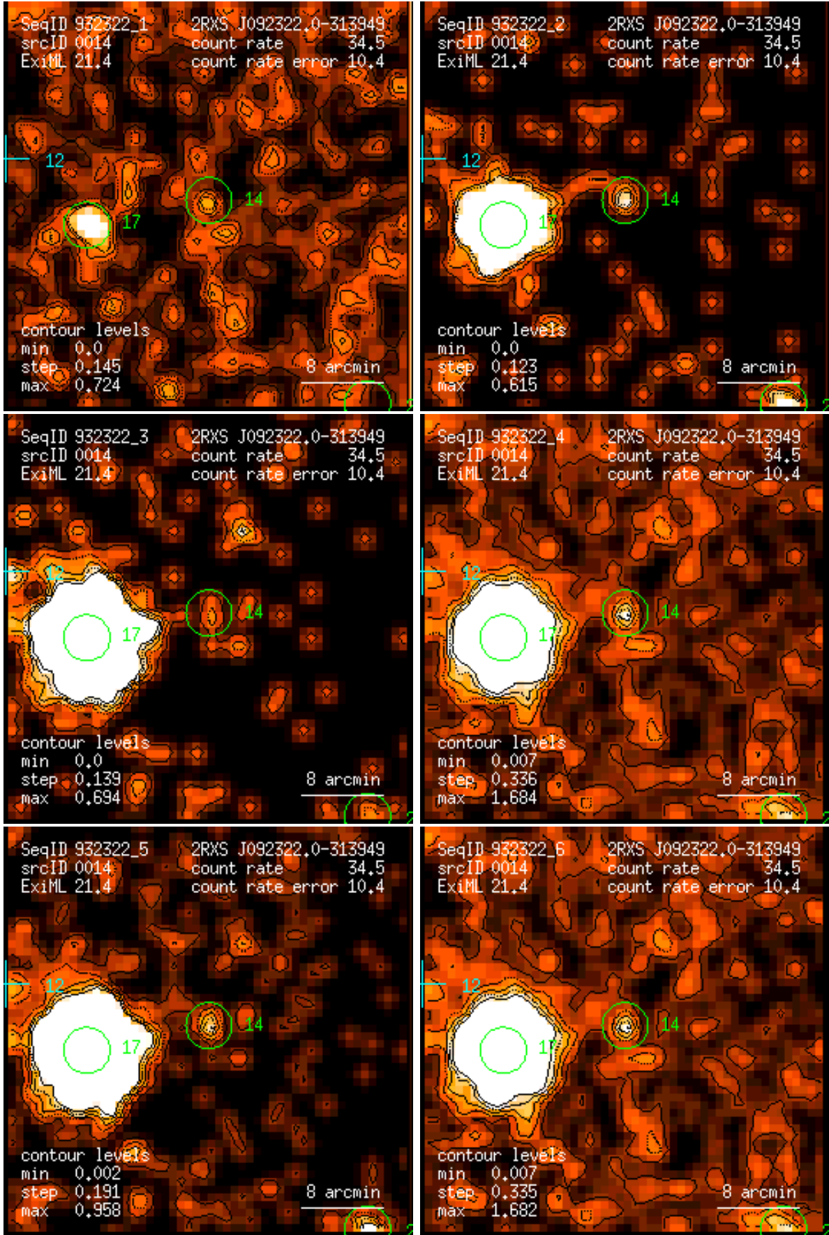
Figure 14: RASS 932322: detection 0014: band rate images, Gaussian filter: (1) PSPC channels 11 – 41, (2) 52 – 90, (3) 91 – 201, (4) 11 – 235, (5) 52 – 201, (6) 11 – 201. Broad band rates in counts/ks. Band rate contour levels in counts/ks/arcmin 2 .
