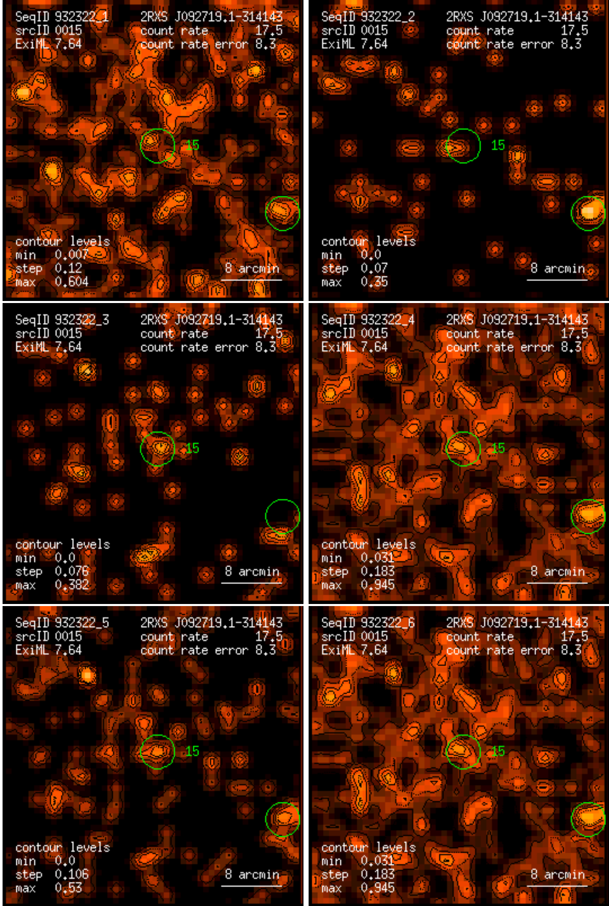
Figure 15: RASS 932322: detection 0015: band rate images, Gaussian filter: (1) PSPC channels 11 – 41, (2) 52 – 90, (3) 91 – 201, (4) 11 – 235, (5) 52 – 201, (6) 11 – 201. Broad band rates in counts/ks. Band rate contour levels in counts/ks/arcmin 2 .
