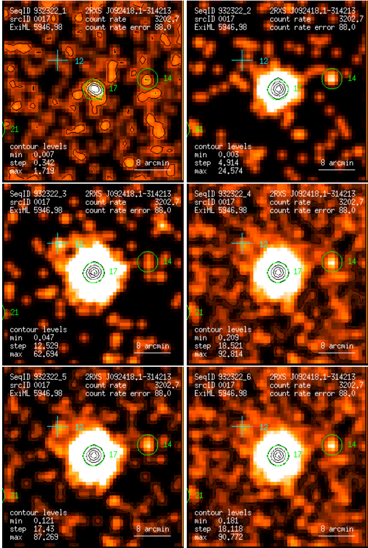
Figure 17: RASS 932322: detection 0017: band rate images, Gaussian filter: (1) PSPC channels 11 – 41, (2) 52 – 90, (3) 91 – 201, (4) 11 – 235, (5) 52 – 201, (6) 11 – 201. Broad band rates in counts/ks. Band rate contour levels in counts/ks/arcmin 2 .
