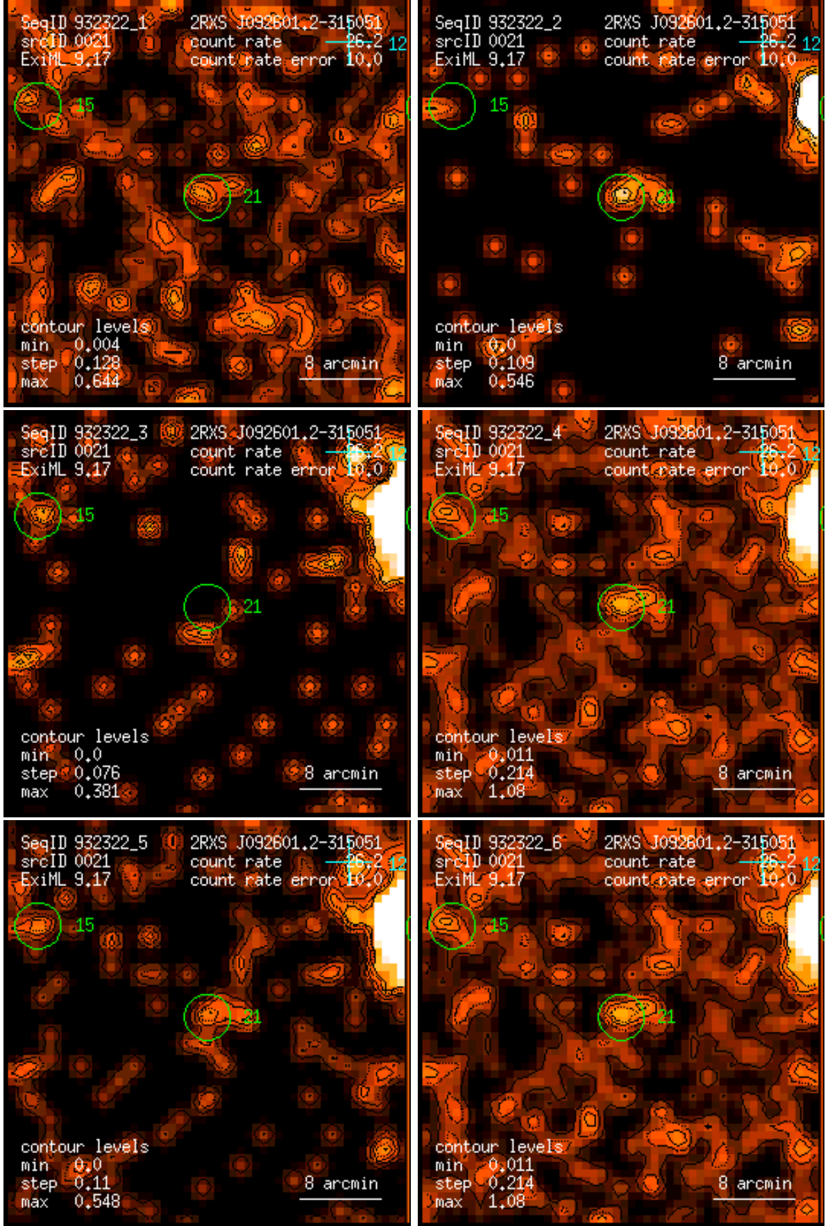
Figure 21: RASS 932322: detection 0021: band rate images, Gaussian filter: (1) PSPC channels 11 – 41, (2) 52 – 90, (3) 91 – 201, (4) 11 – 235, (5) 52 – 201, (6) 11 – 201. Broad band rates in counts/ks. Band rate contour levels in counts/ks/arcmin 2 .
