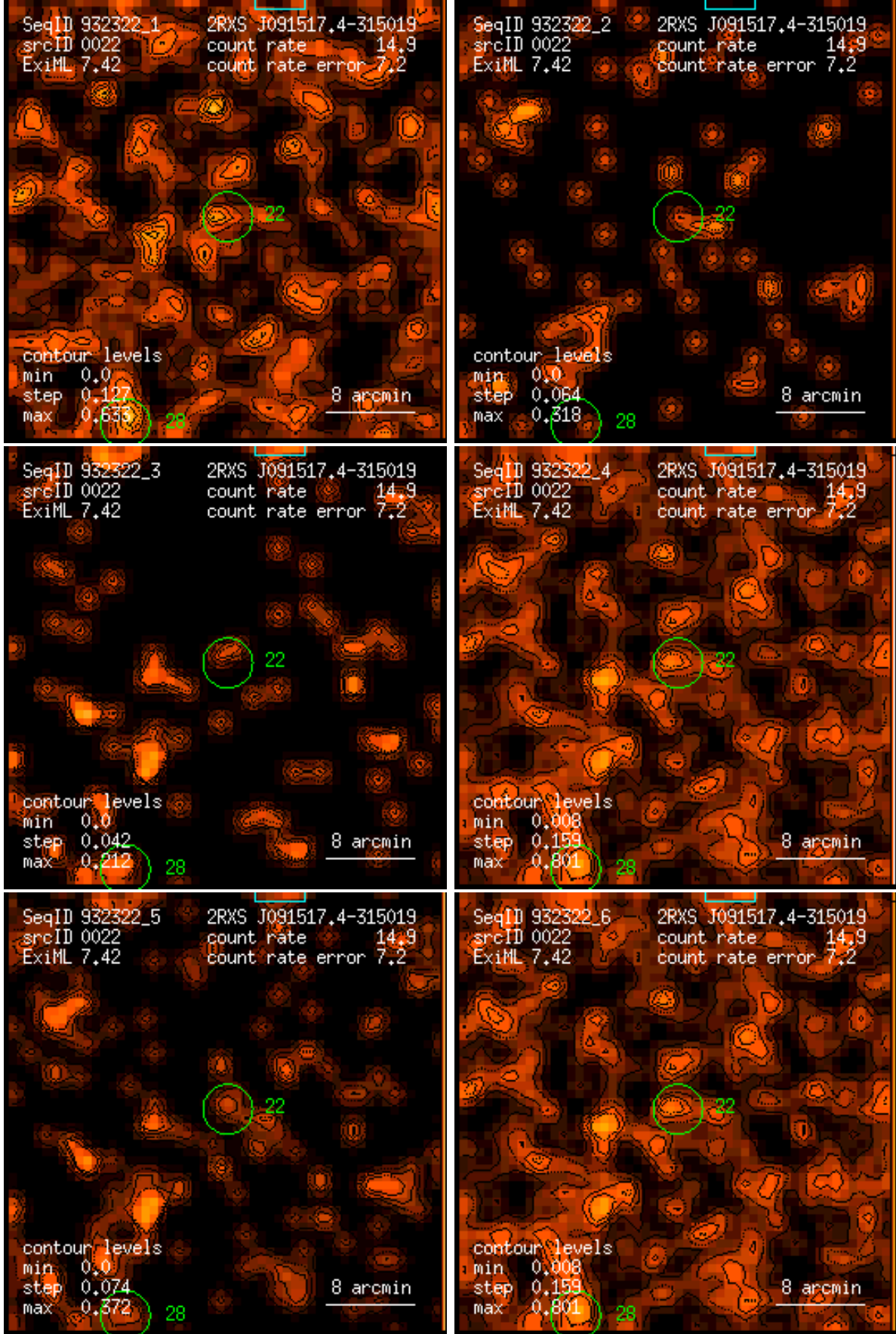
Figure 22: RASS 932322: detection 0022: band rate images, Gaussian filter: (1) PSPC channels 11 – 41, (2) 52 – 90, (3) 91 – 201, (4) 11 – 235, (5) 52 – 201, (6) 11 – 201. Broad band rates in counts/ks. Band rate contour levels in counts/ks/arcmin 2 .
