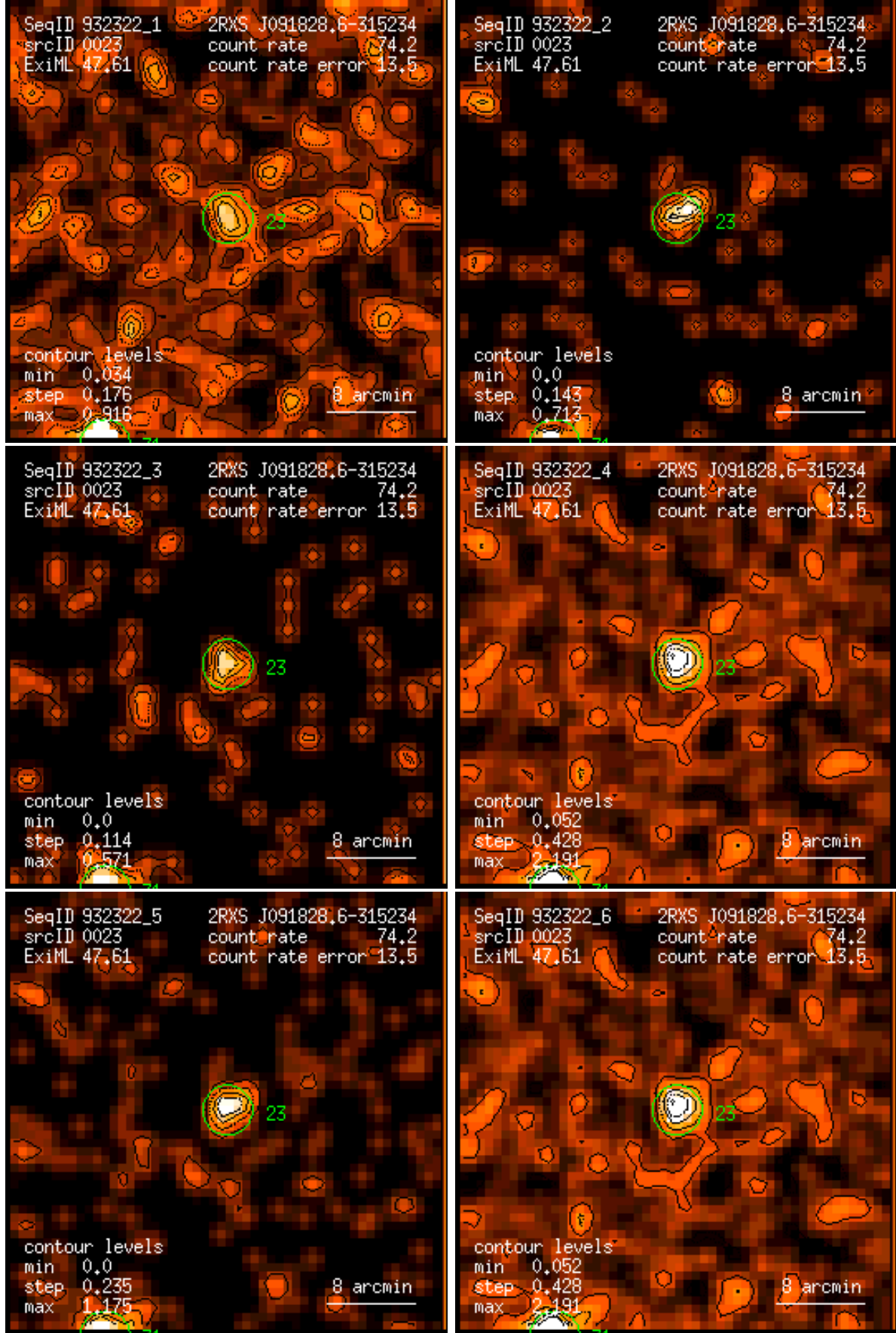
Figure 23: RASS 932322: detection 0023: band rate images, Gaussian filter: (1) PSPC channels 11 – 41, (2) 52 – 90, (3) 91 – 201, (4) 11 – 235, (5) 52 – 201, (6) 11 – 201. Broad band rates in counts/ks. Band rate contour levels in counts/ks/arcmin 2 .
