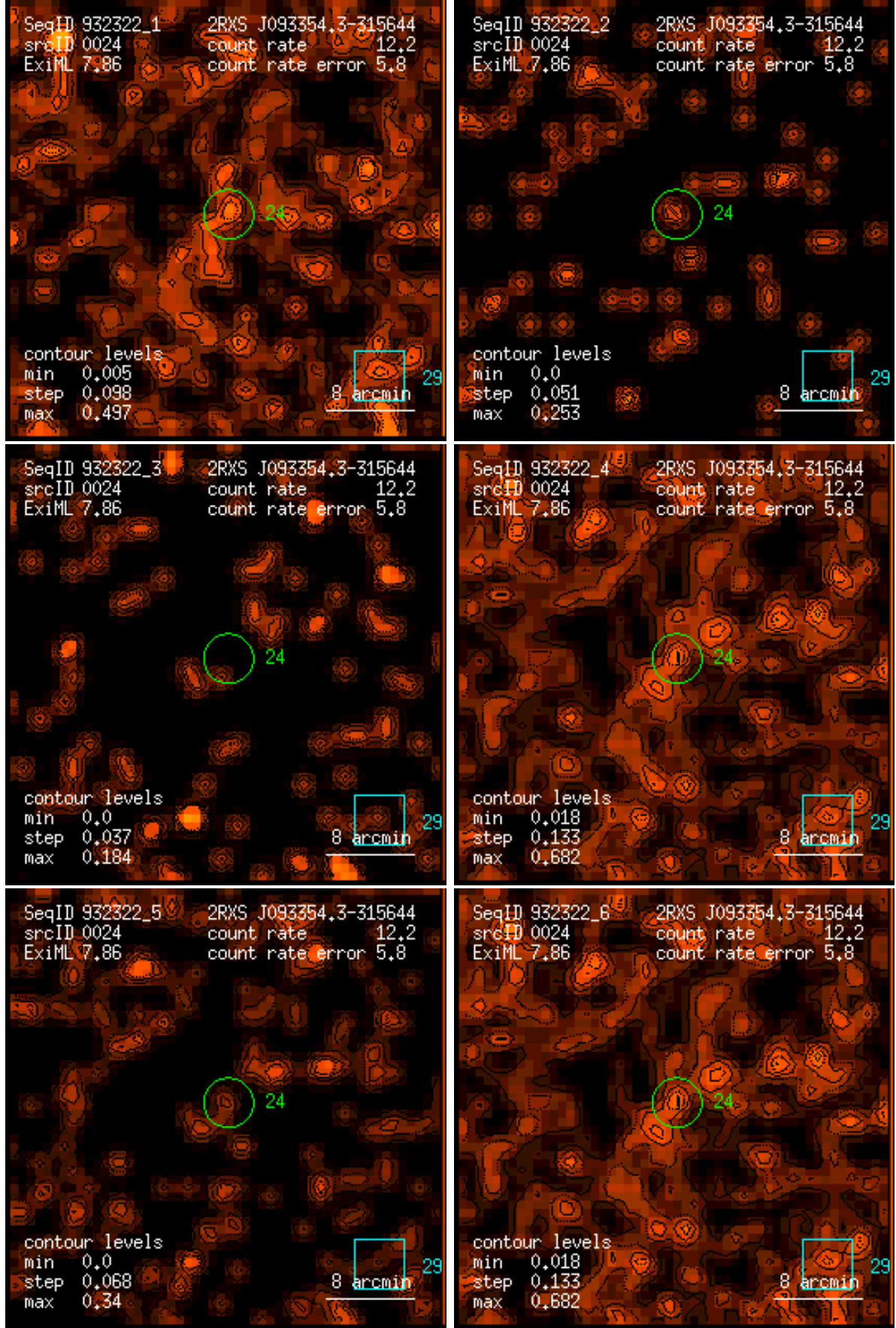
Figure 24: RASS 932322: detection 0024: band rate images, Gaussian filter: (1) PSPC channels 11 – 41, (2) 52 – 90, (3) 91 – 201, (4) 11 – 235, (5) 52 – 201, (6) 11 – 201. Broad band rates in counts/ks. Band rate contour levels in counts/ks/arcmin 2 .
