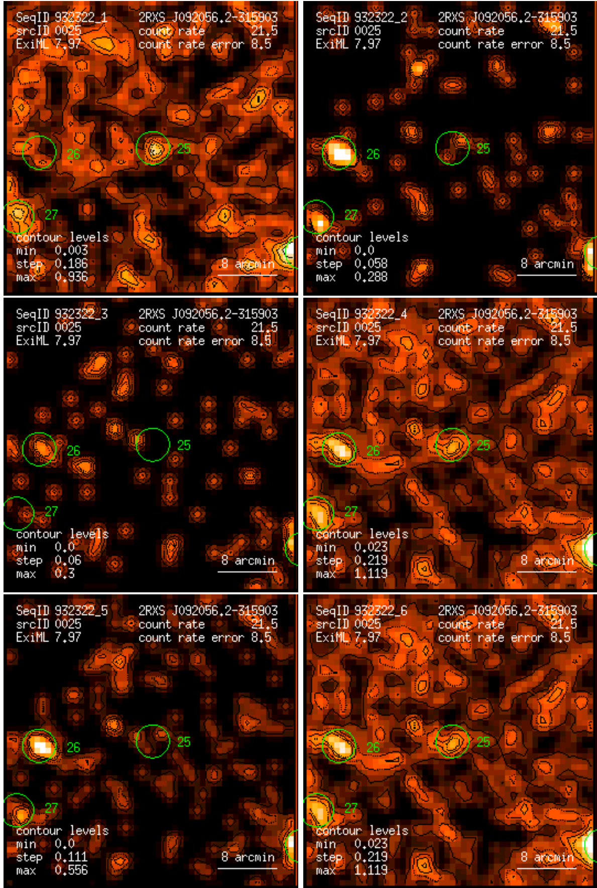
Figure 25: RASS 932322: detection 0025: band rate images, Gaussian filter: (1) PSPC channels 11 – 41, (2) 52 – 90, (3) 91 – 201, (4) 11 – 235, (5) 52 – 201, (6) 11 – 201. Broad band rates in counts/ks. Band rate contour levels in counts/ks/arcmin 2 .
