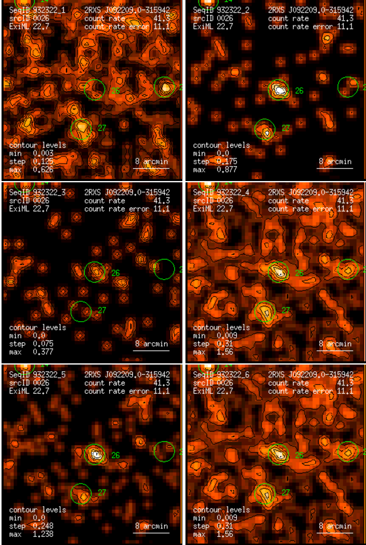
Figure 26: RASS 932322: detection 0026: band rate images, Gaussian filter: (1) PSPC channels 11 – 41, (2) 52 – 90, (3) 91 – 201, (4) 11 – 235, (5) 52 – 201, (6) 11 – 201. Broad band rates in counts/ks. Band rate contour levels in counts/ks/arcmin 2 .
