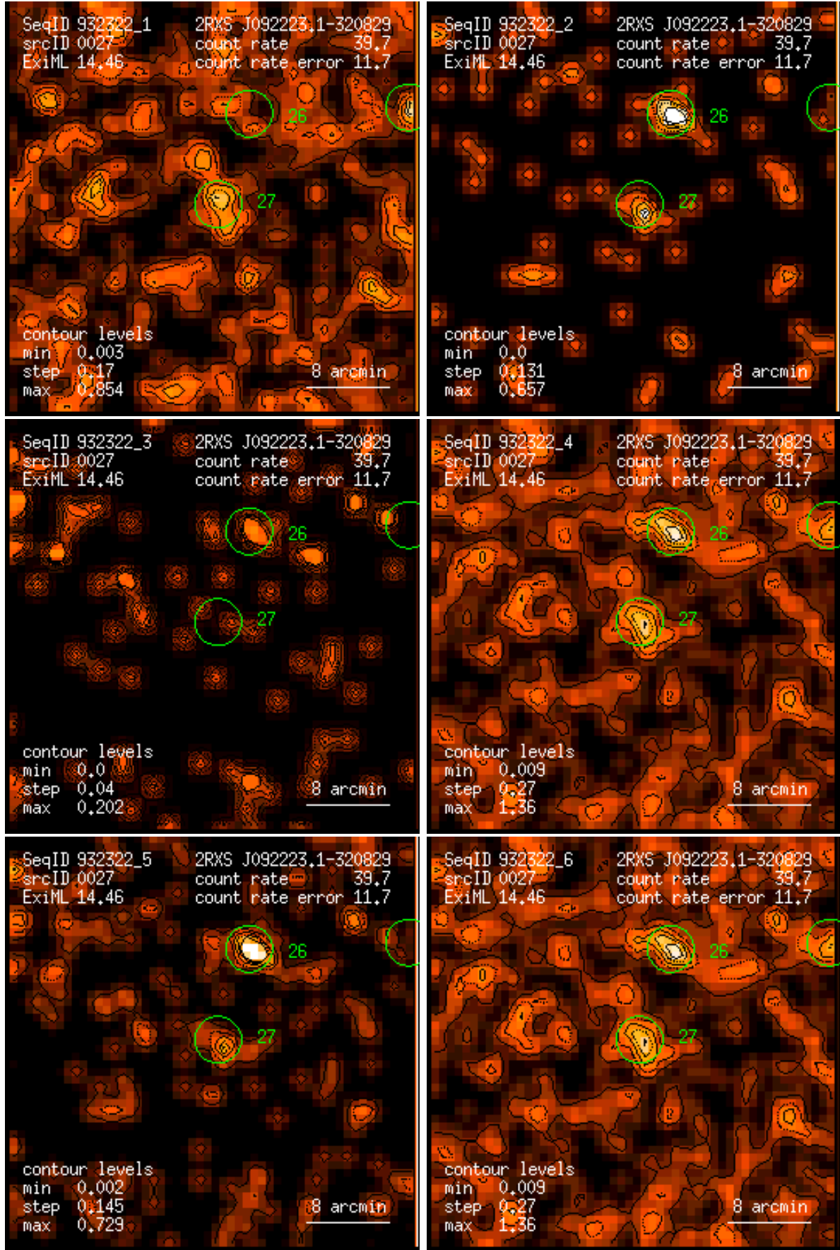
Figure 27: RASS 932322: detection 0027: band rate images, Gaussian filter: (1) PSPC channels 11 – 41, (2) 52 – 90, (3) 91 – 201, (4) 11 – 235, (5) 52 – 201, (6) 11 – 201. Broad band rates in counts/ks. Band rate contour levels in counts/ks/arcmin 2 .
