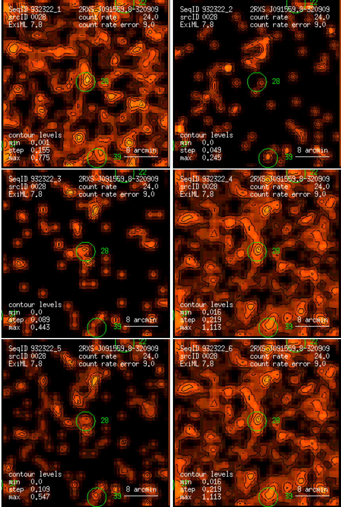
Figure 28: RASS 932322: detection 0028: band rate images, Gaussian filter: (1) PSPC channels 11 – 41, (2) 52 – 90, (3) 91 – 201, (4) 11 – 235, (5) 52 – 201, (6) 11 – 201. Broad band rates in counts/ks. Band rate contour levels in counts/ks/arcmin 2 .
