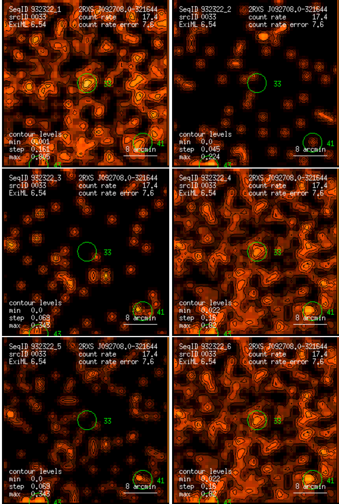
Figure 33: RASS 932322: detection 0033: band rate images, Gaussian filter: (1) PSPC channels 11 – 41, (2) 52 – 90, (3) 91 – 201, (4) 11 – 235, (5) 52 – 201, (6) 11 – 201. Broad band rates in counts/ks. Band rate contour levels in counts/ks/arcmin 2 .
