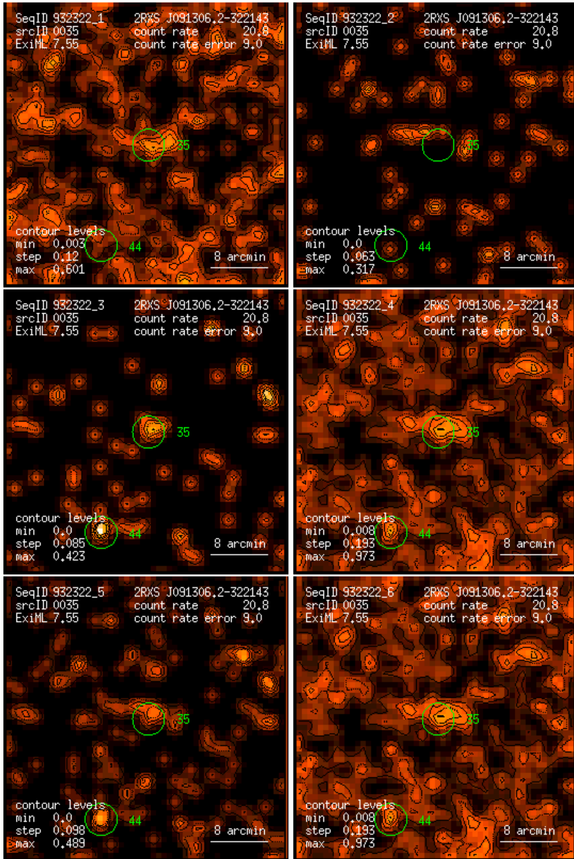
Figure 35: RASS 932322: detection 0035: band rate images, Gaussian filter: (1) PSPC channels 11 – 41, (2) 52 – 90, (3) 91 – 201, (4) 11 – 235, (5) 52 – 201, (6) 11 – 201. Broad band rates in counts/ks. Band rate contour levels in counts/ks/arcmin 2 .
