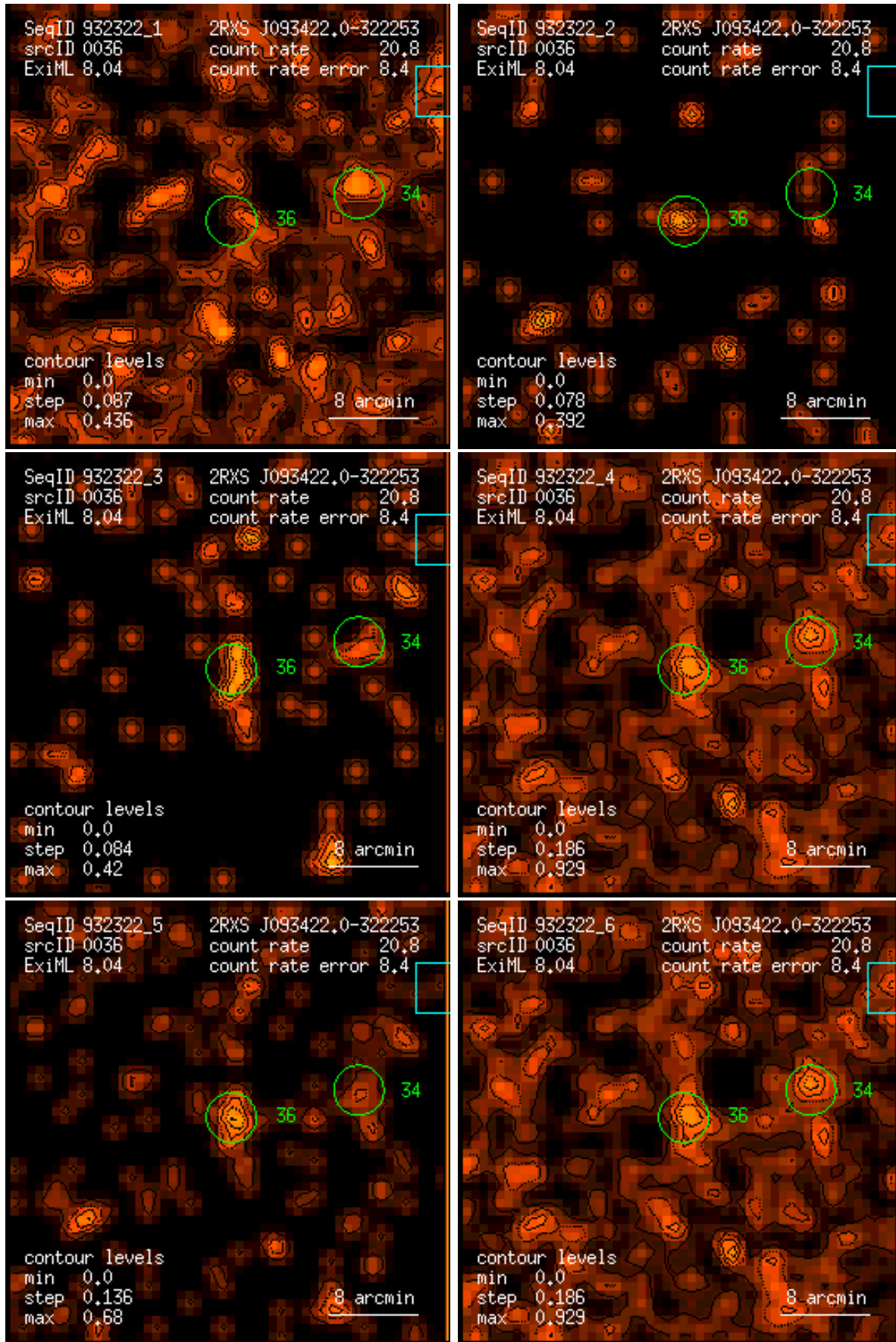
Figure 36: RASS 932322: detection 0036: band rate images, Gaussian filter: (1) PSPC channels 11 – 41, (2) 52 – 90, (3) 91 – 201, (4) 11 – 235, (5) 52 – 201, (6) 11 – 201. Broad band rates in counts/ks. Band rate contour levels in counts/ks/arcmin 2 .
