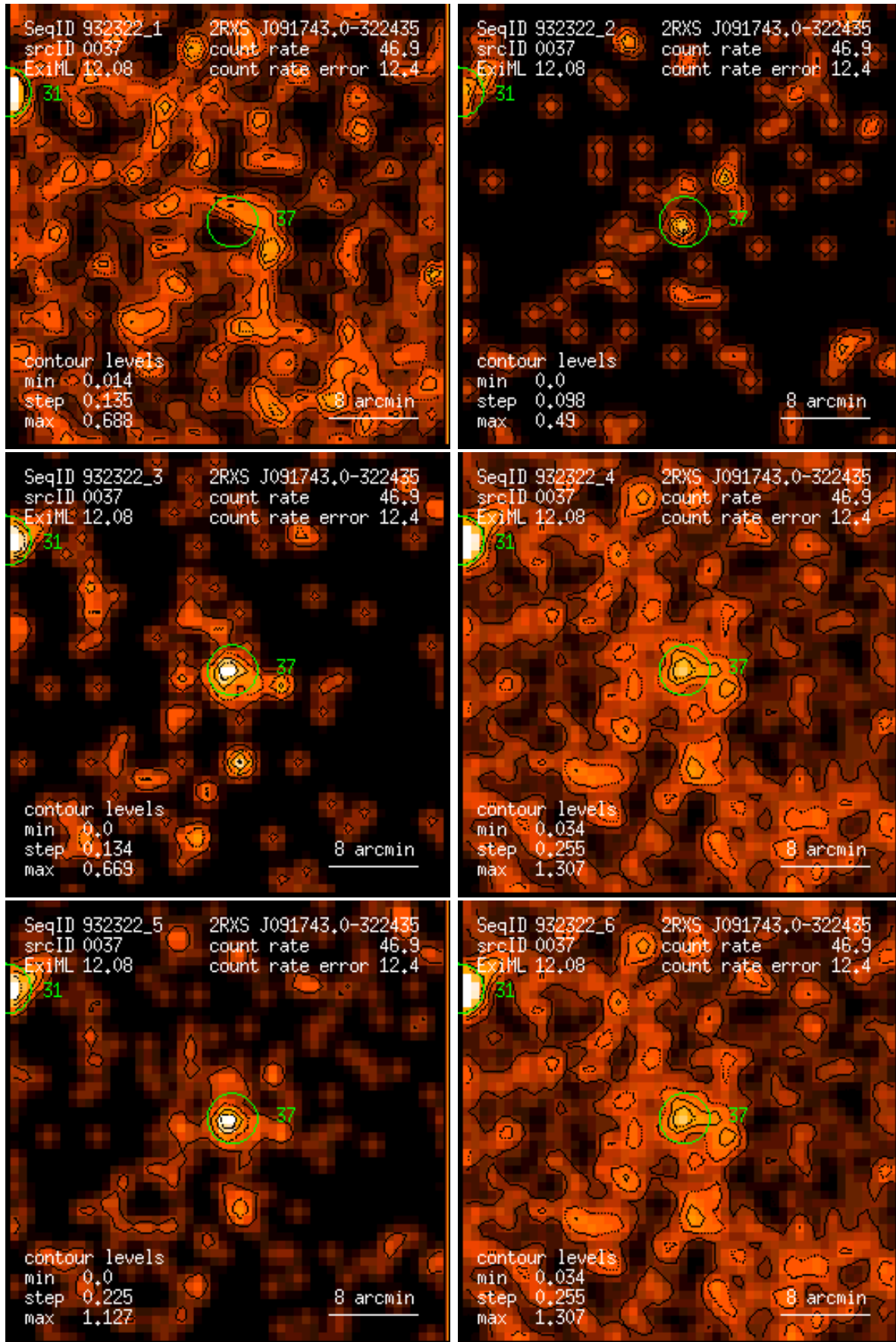
Figure 37: RASS 932322: detection 0037: band rate images, Gaussian filter: (1) PSPC channels 11 – 41, (2) 52 – 90, (3) 91 – 201, (4) 11 – 235, (5) 52 – 201, (6) 11 – 201. Broad band rates in counts/ks. Band rate contour levels in counts/ks/arcmin 2 .
